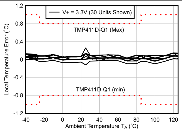
Figure 9-9. Local Temperature Error vs TMP411D-Q1 Ambient Temperature
