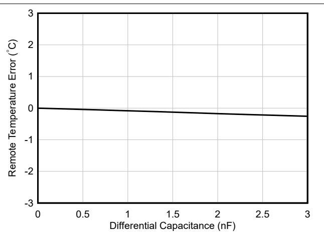
Figure 6-28. Remote Temperature Error vs Differential Capacitance
