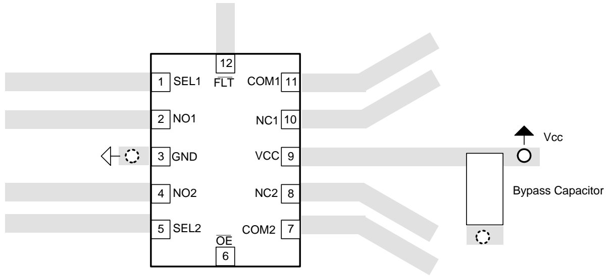
Figure 20. Layout Example
