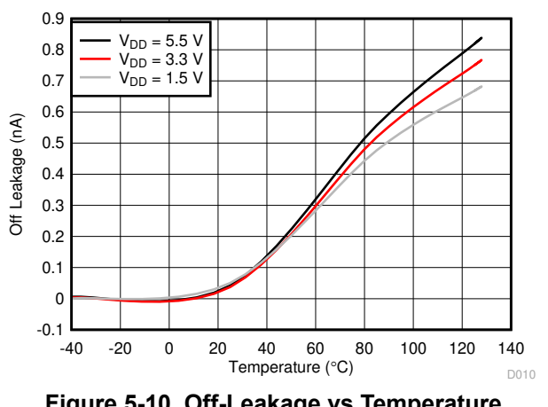
Figure 5-10. Off-Leakage vs Temperature
