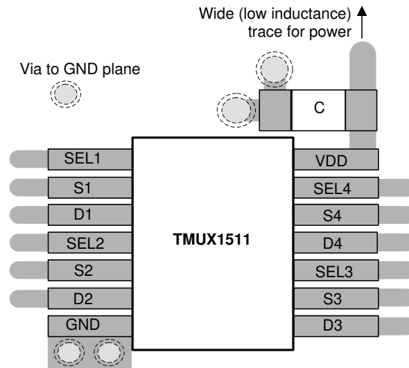
Figure 10-3. Example Layout
