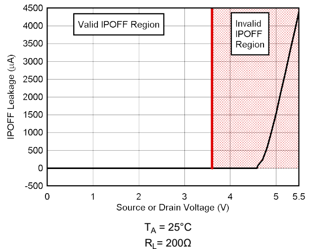
Figure 5-14. IPOFF Leakage vs Source or Drain Voltage
