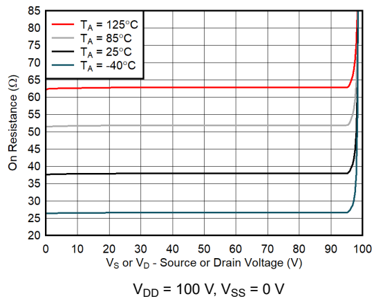
Figure 7-9. On-Resistance vs Source or Drain Voltage
