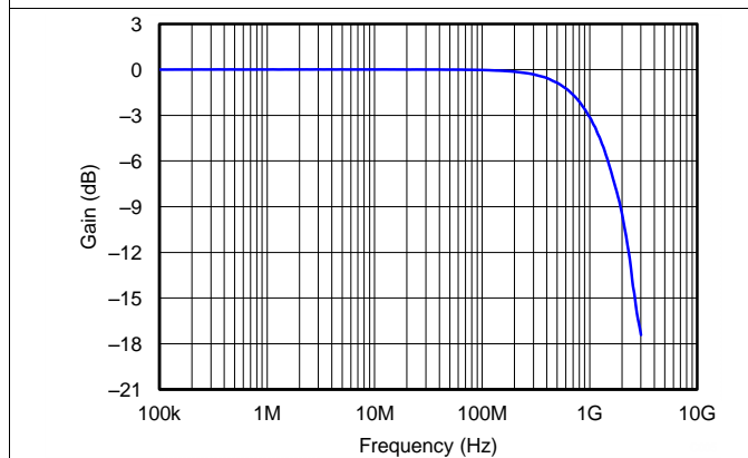
Figure 5. Utility Pin Insertion Loss
