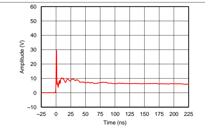
Figure 6. Utility Pin, +8kv IEC Voltage Clamp Waveform
