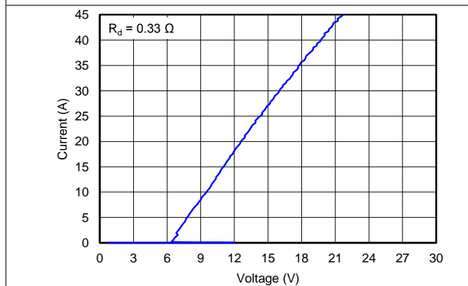
Figure 3. Utility Pin TLP Curve
