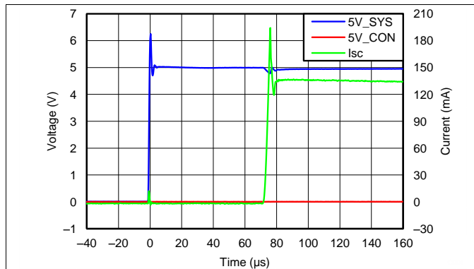
Figure 1. Power up to Short Circuit
