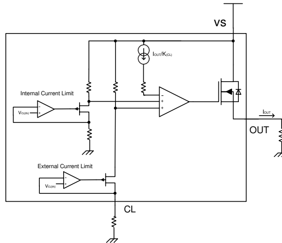
Figure 6-1. Current Limit
