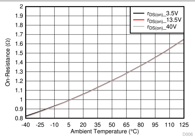
Figure 5-8. FET On-Resistance
