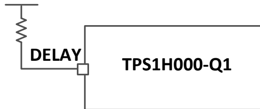
Figure 6-6. Auto-Retry-Mode Connection
