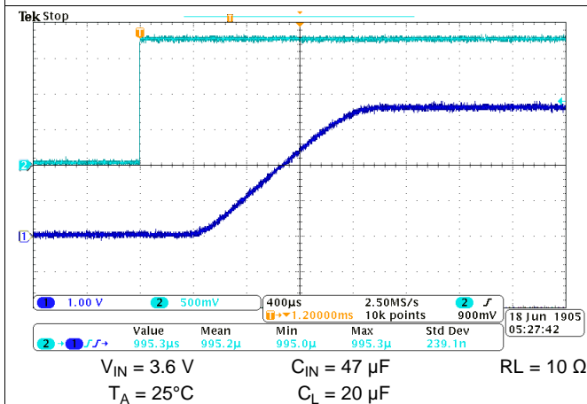
Figure 22. Turn-On Response
