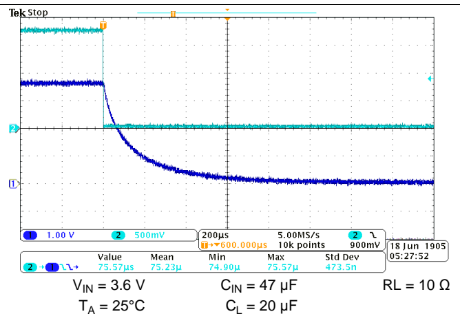
Figure 23. Turn-Off Response
