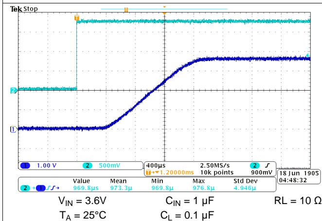
Figure 20. Turn-On Response
