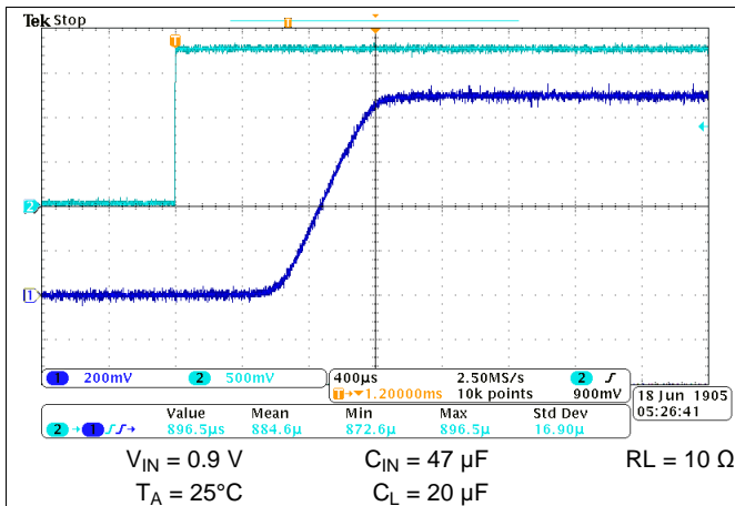
Figure 18. Turn-On Response
