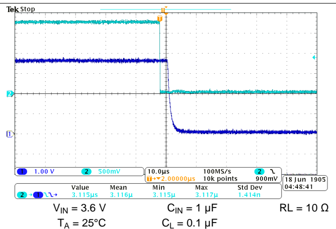
Figure 21. Turn-Off Response
