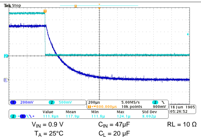
Figure 19. Turn-Off Response
