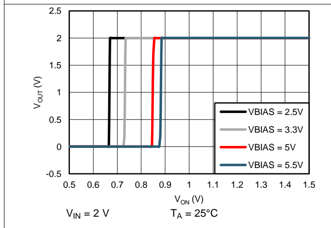
Figure 11. Output Voltage vs ON Voltage
