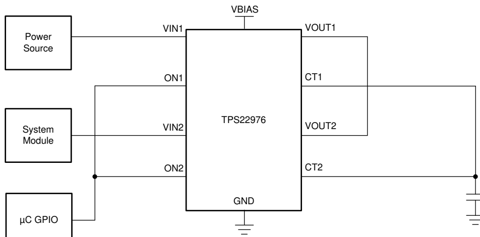
Figure 9-4. Reverse Current Blocking
