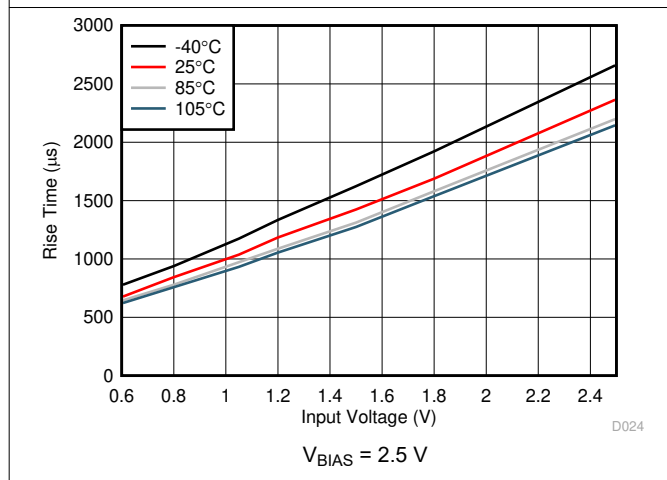
Figure 6-29. Rise Time vs Input Voltage
