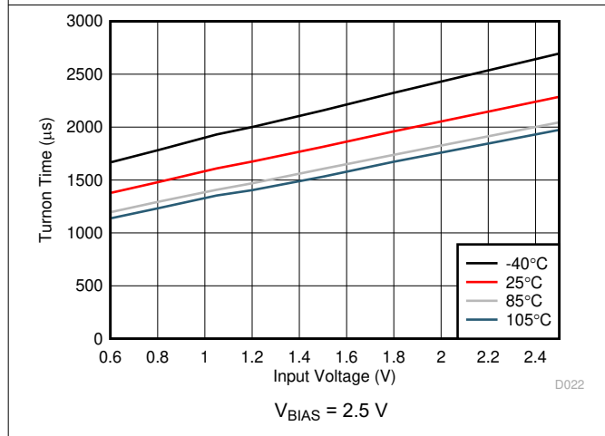
Figure 6-27. Turnon Time vs Input Voltage
