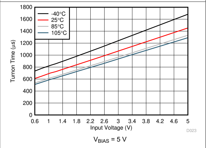
Figure 6-28. Turnon Time vs Input Voltage
