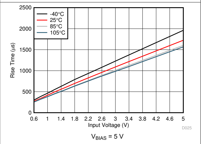
Figure 6-30. Rise Time vs Input Voltage
