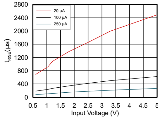
Figure 5-12. Rise Time vs Input Voltage with Different I_{\text{ON}}
