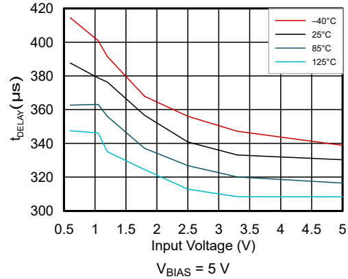
Figure 5-6. Delay Time vs Input Voltage
