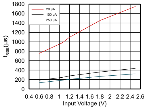
Figure 5-11. Rise Time vs Input Voltage with Different I_{\text{ON}}
