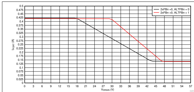
Figure 9-79. 1x Mode (2xFBn = 0) Foldback Curves, I PORT vs V DRAIN
