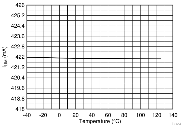
Figure 7-24. 1x Mode ( 2x\text{FBn} = 0 ) Current Limit vs Temperature
