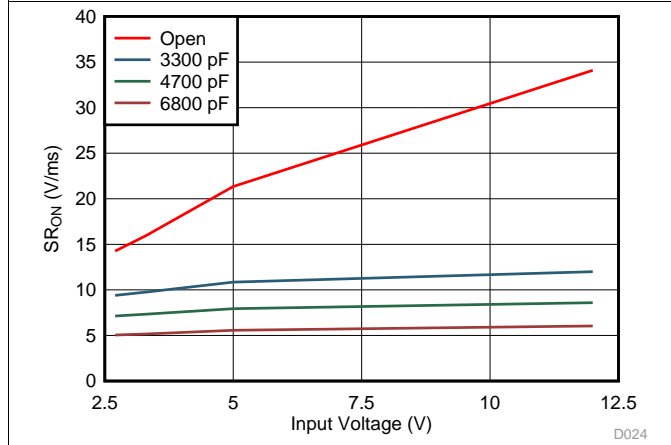
Different C_{dV/dt} values D024
