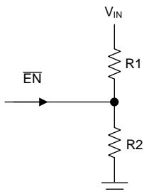
Figure 48. Overtoltage Lockout
