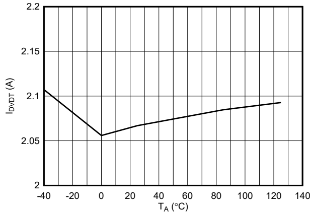
Figure 7-15. DVDT Charging Current Across Temperature
