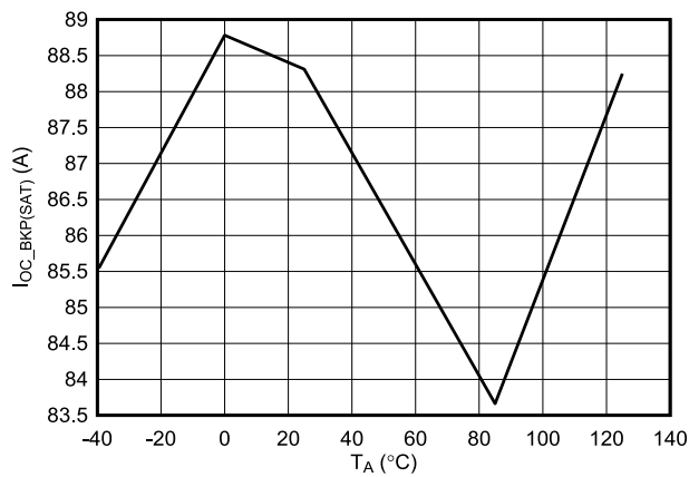
Figure 7-9. ackup Overcurrent Protection Threshold (Start-up) Accuracy
