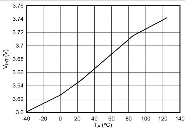
Figure 7-11. ITIMER Pin Internal Pullup Voltage Across Temperature
