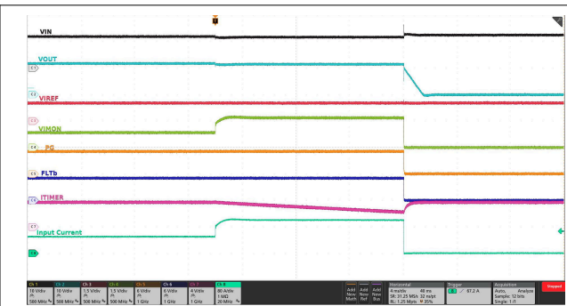
Figure 7-32. Overcurrent Protection Response (Circuit-Breaker)
