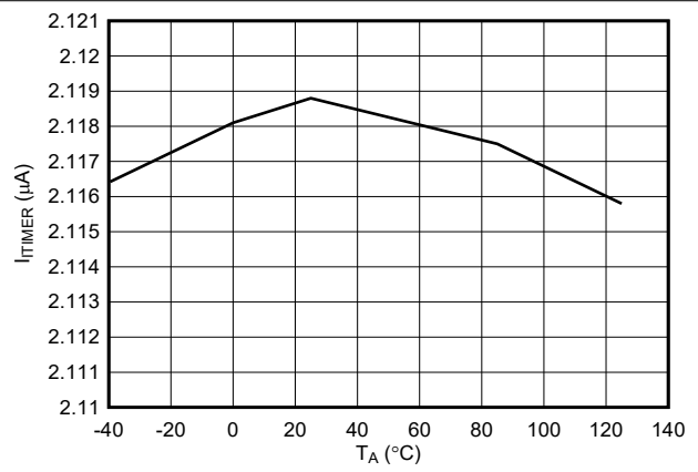
Figure 7-12. ITIMER Pin Discharge Current Across Temperature
