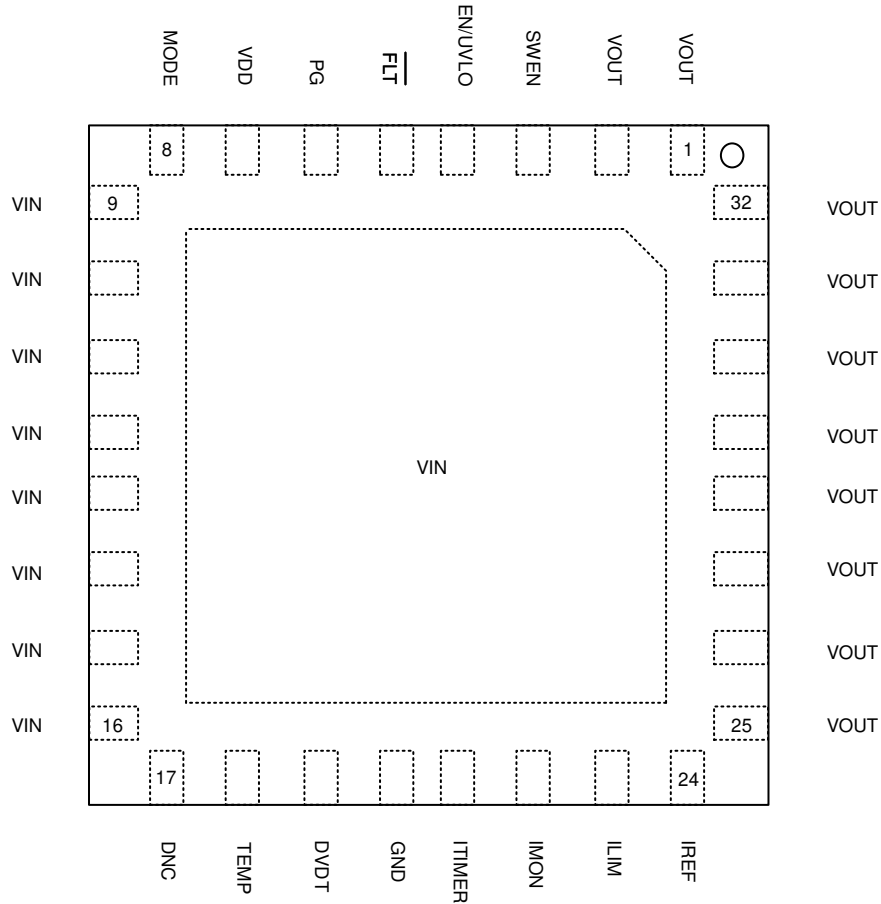
Figure 6-1. TPS25984x RZJ Package 32-pin QFN Top View
