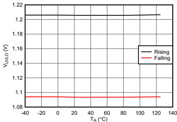
Figure 7-5. EN/UVLO Thresholds For FET Turn-off Across Temperature
