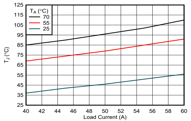
Figure 7-18. Junction Temperature vs Load Current (No Air-Flow)
