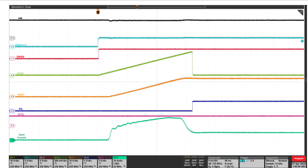
Figure 9-7. Start-up with EN/UVLO: V_{IN} = 12 V, EN/UVLO Stepped Up From 0 V to 3 V, C_{LOAD} = 50 mF, R_{LOAD(Start-up)} = 0.48 \Omega , C_{DVRT} = 33 nF, and R_{ILIM} on Each Device = 442 \Omega
