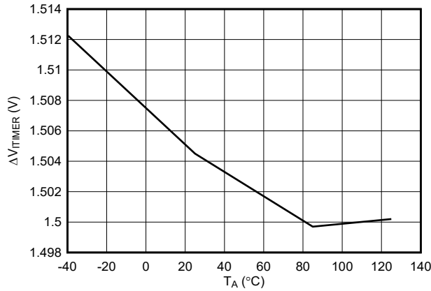
Figure 7-13. ITIMER Pin Discharge Differential Voltage Threshold Across Temperature
