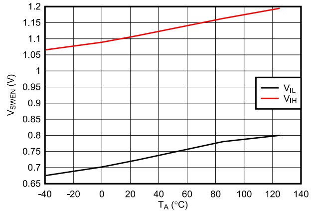
Figure 7-14. SWEN Pin Logic Thresholds Across Temperature
