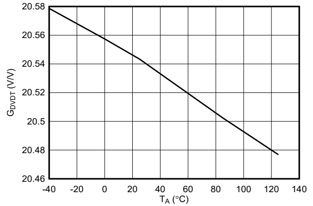
Figure 7-16. DVDT Gain Across Temperature
