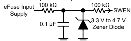
Figure 9-14. Zener Regulator Used as Pullup Supply for SWEN
