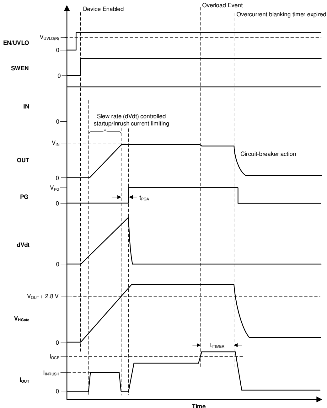
Figure 8-8. TPS25984x PG Timing Diagram
