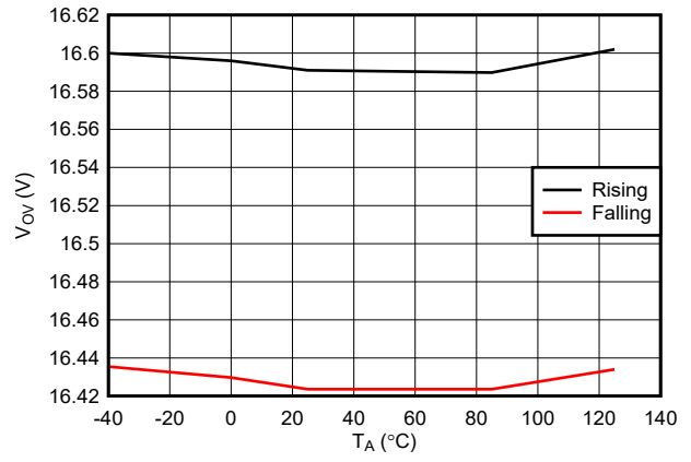
Figure 7-4. VIN Overvoltage Protection Thresholds Across Temperature
