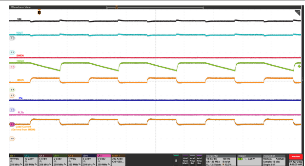
Figure 9-9. Transient Overload: V_{IN} = 12 V, C_{TIMER} = 22 nF, C_{LOAD} = 50 mF, R_{IMON} = 200 \Omega , R_{REF} = 40.2 k \Omega , and Load Current Stepped from 250 A to 300 A then 250 A within 10 ms
