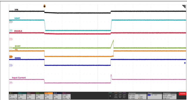
Figure 7-26. Power Up and Down Sequencing Using SWEN Pin
