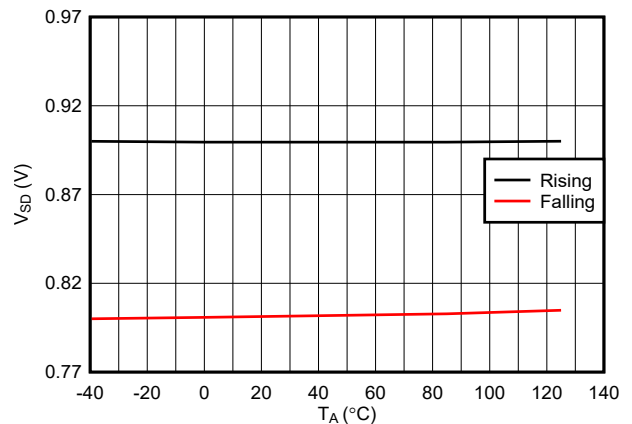
Figure 7-6. EN/UVLO Based Thresholds for Device Shutdown Across Temperature
