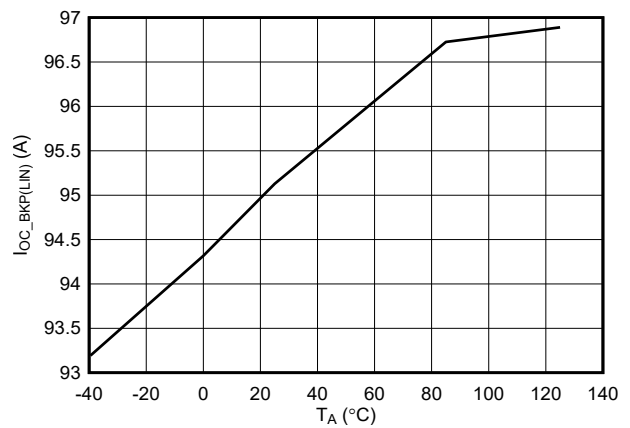
Figure 7-10. Backup Overcurrent Protection Threshold (Steady-State) Accuracy
