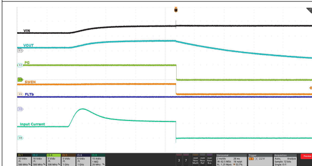
Figure 7-29. Input Overvoltage Protection Response
