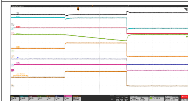
Figure 9-10. Circuit-Breaker Response: V_{IN} = 12 V, C_{TIMER} = 22 nF, C_{LOAD} = 50 mF, R_{IMON} = 200 \Omega , R_{REF} = 40.2 k \Omega , and Load Current Stepped up From 250 A to 400 A for > 20 ms
