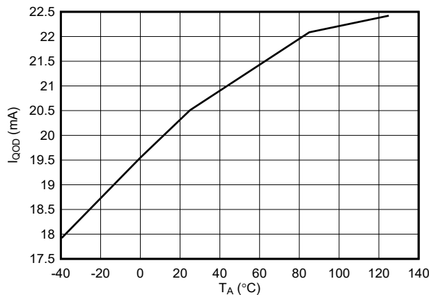
Figure 7-17. QOD Sink Current Across Temperature
