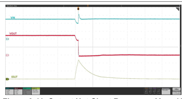
Figure 9-11. Output Hot-Short Response: V_{IN} = 12 V, R_{IMON} = 200 \Omega , R_{REF} = 40.2 k \Omega , and OUT Shorted to GND
