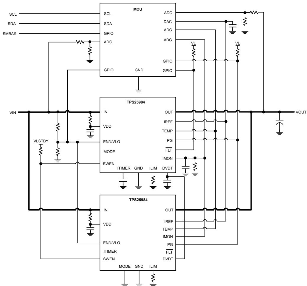
Figure 9-4. Digital Telemetry Using External Microcontroller
