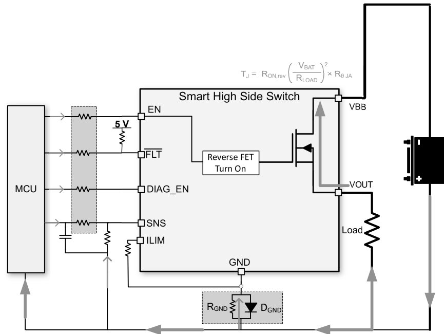
Figure 8-41. Reverse Protection with GND Network
