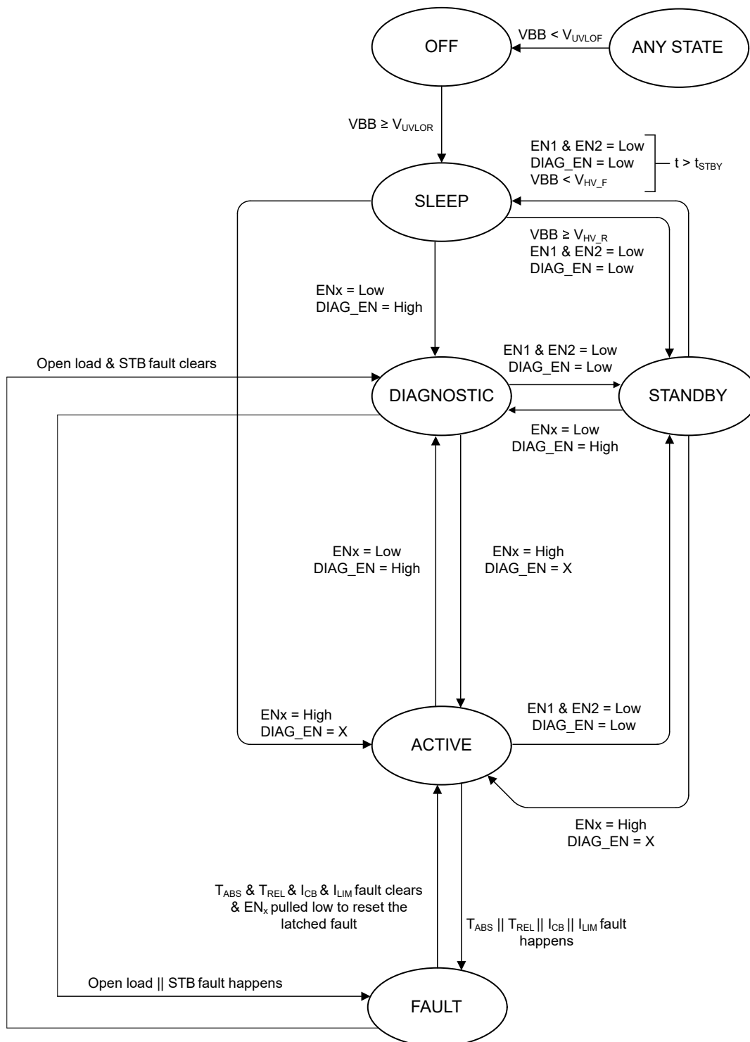
Figure 8-43. State Diagram
