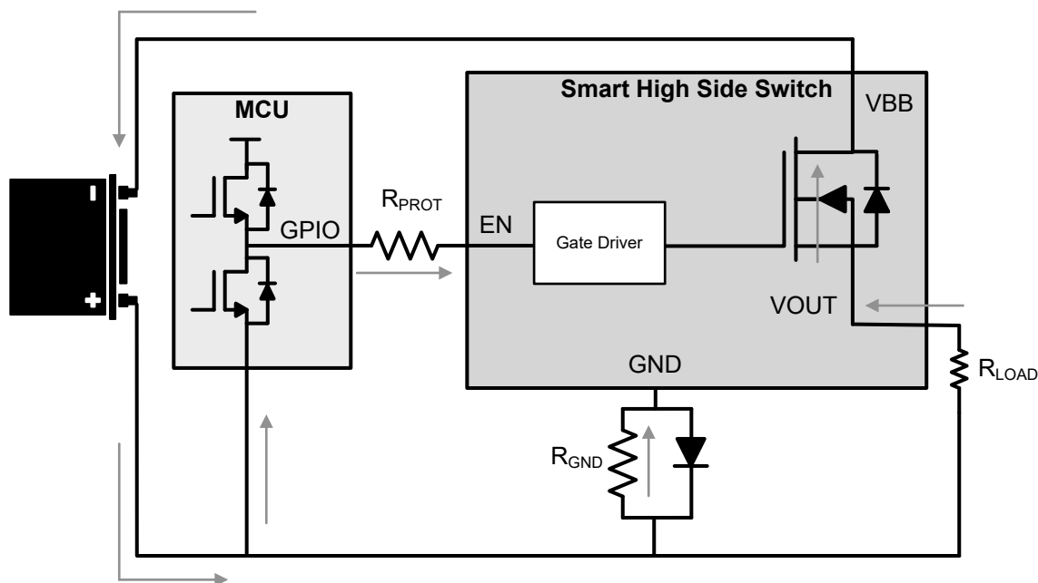
Figure 8-36. Reverse Battery Circuit
