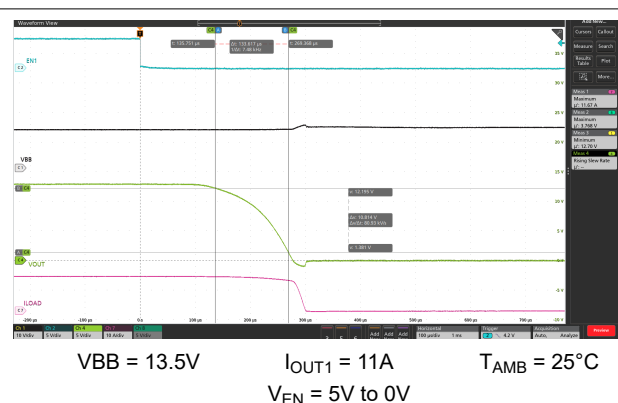
Figure 9-6. Falling Slew Rate (D, B version)
