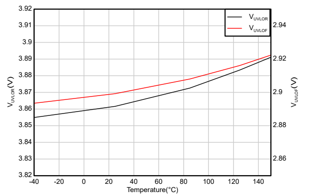
Figure 6-36. Undervoltage Lockout Thresholds ( V_{UVLOR} , V_{UVLOF} ) vs Temperature
