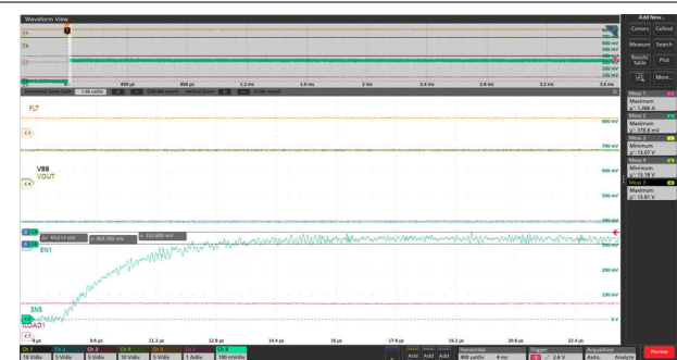
Figure 8-11. SNS Pin Ripple With 150pF C_{SNS} at V_{BS} = 13.5V , I_{LIM} = OPEN , R_L = 10\Omega , R_{SNS} = 1k\Omega and T_A = 25^\circ C
