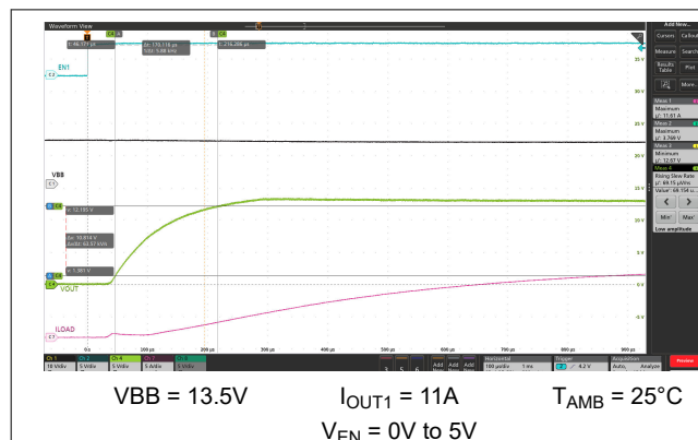
Figure 9-5. Rising Slew Rate (D, B version)
