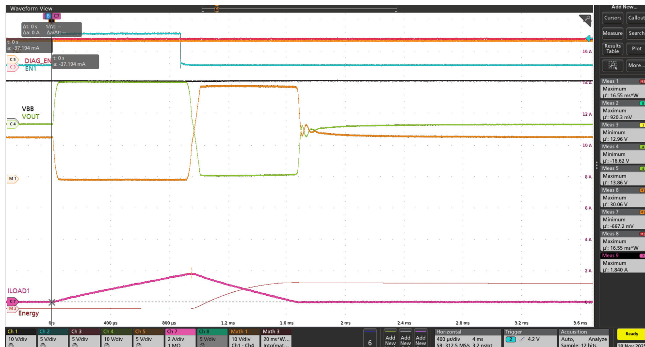
Figure 8-26. 5mH Inductive Load Driving (VBB = 13.5V, T_{AMB} = 125°C)
