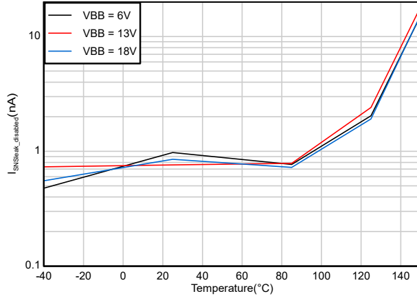
Figure 6-7. I_{SNS} leakage with Diagnostics disabled vs Temperature
