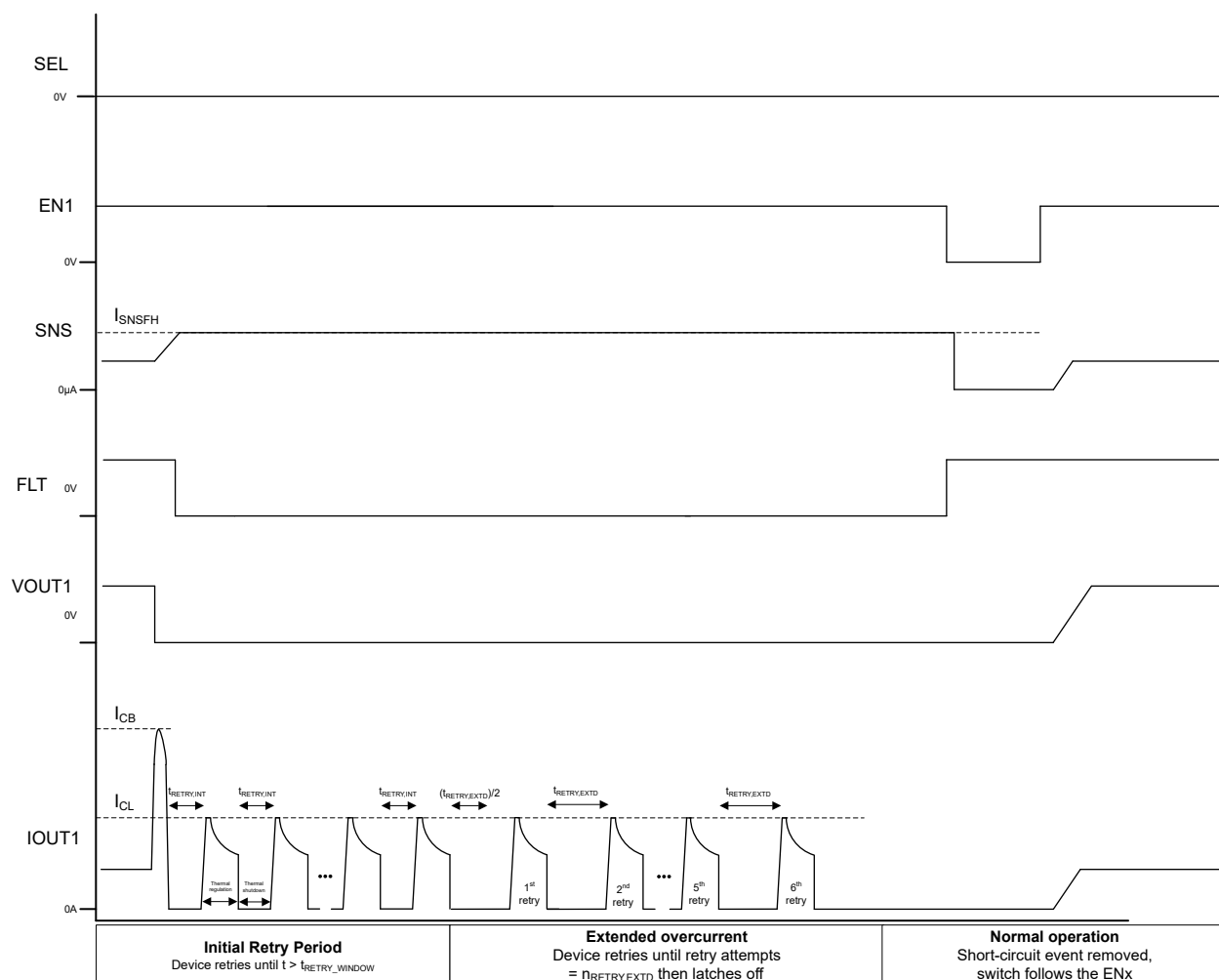
Figure 8-21. Retry Behavior After Hot-Short with Thermal Regulation
