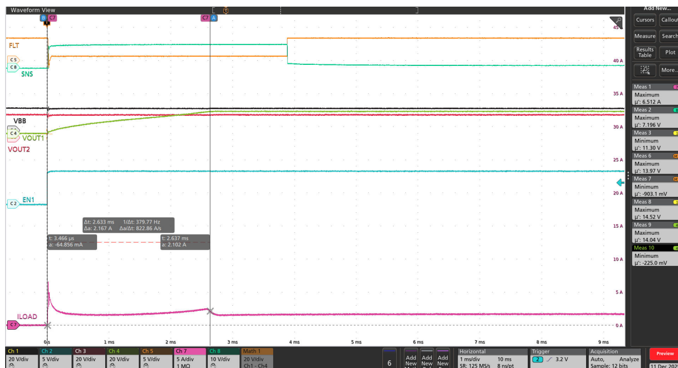
Figure 8-30. 220uF Capacitive Load Charging with Channel 1 of TPS2HC16-Q1 Device at 13.5V VBB, ILIM Pin OPEN and 125°C Ambient Temperature (no load on channel 2)
