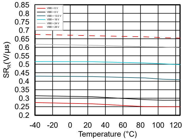
Figure 6-13. SR R vs Temperature Over V BB Voltage
