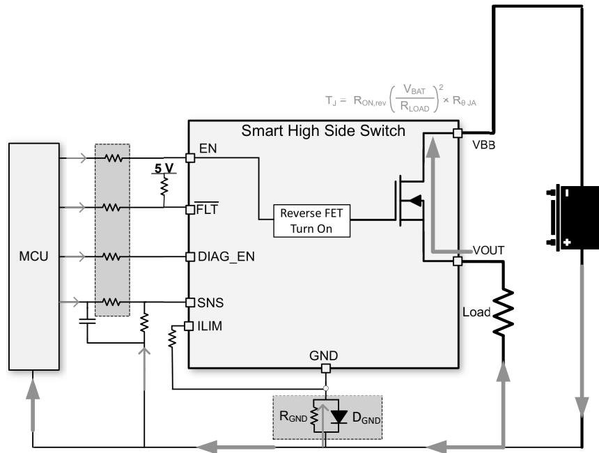
Figure 7-22. Reverse Protection With GND Network
