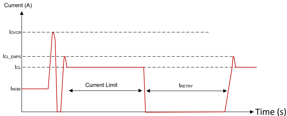
Figure 7-9. Hot Short Event (auto-retry version)
