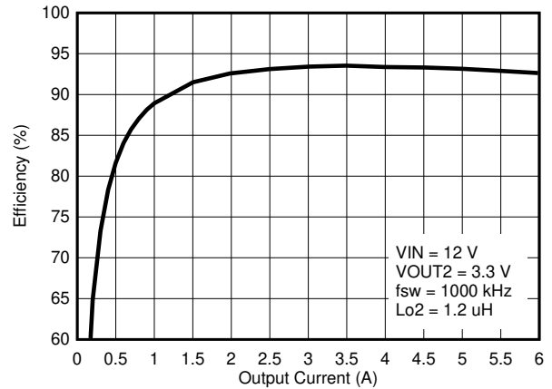
Figure 8-4. V OUT2 Efficiency
