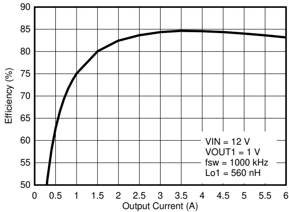
Figure 8-3. V OUT1 Efficiency
