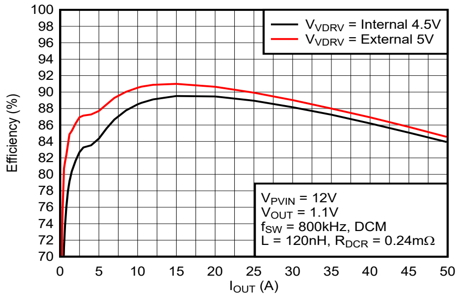
Typical Efficiency
