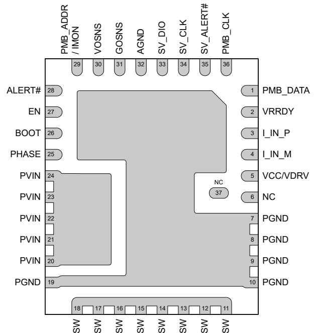
Figure 4-2. RXX 37-Pin WQFN-FCRLF Package (Bottom View)
