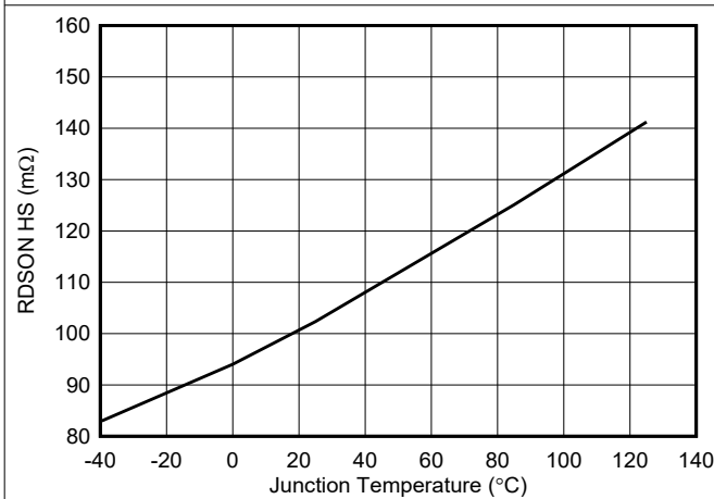
Figure 5-5. Low-Side Rdson
