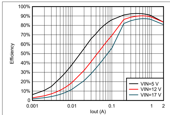
Figure 5-13. TPS562206 Efficiency at 1.05 Vout With 2.2uH Inductor
