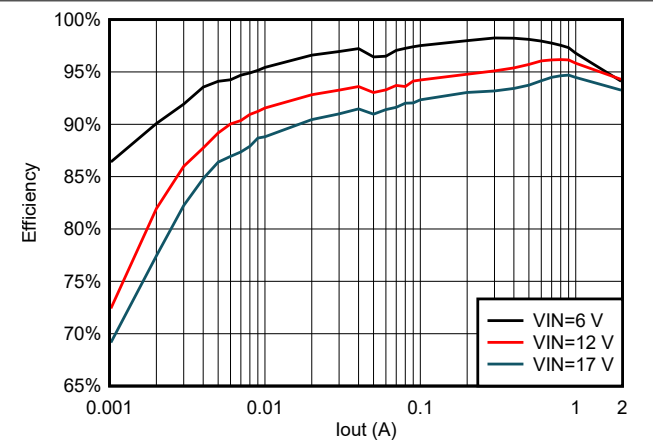
Figure 5-16. TPS562203 Efficiency at 5 Vout With 4.7uH Inductor
