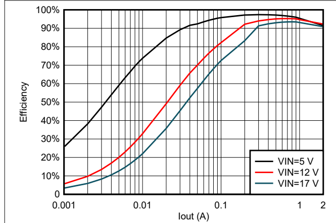
Figure 5-15. TPS562206 Efficiency at 3.3 Vout With 4.7uH Inductor
