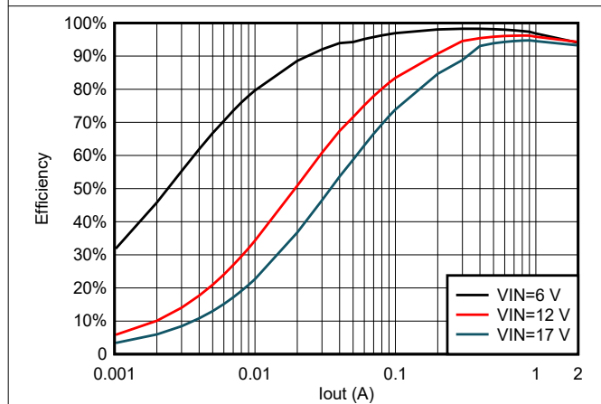
Figure 5-17. TPS562206 Efficiency at 5 Vout With 4.7uH Inductor
