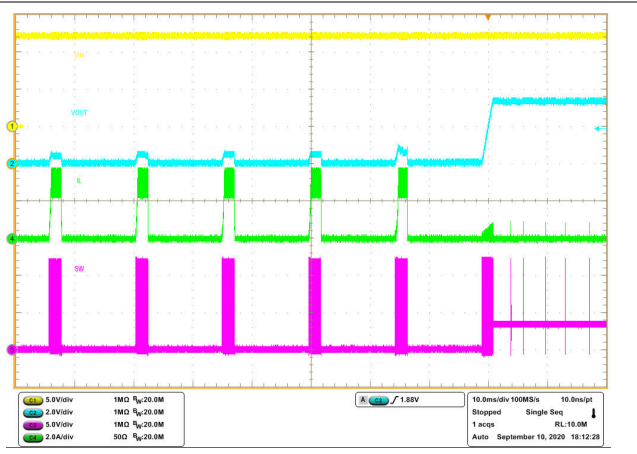
Figure 8-21. Output Short Recovery
