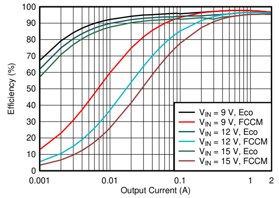
Figure 6-16. V_{OUT} = 7\text{-V} Efficiency, L = 5.6\ \mu\text{H}
