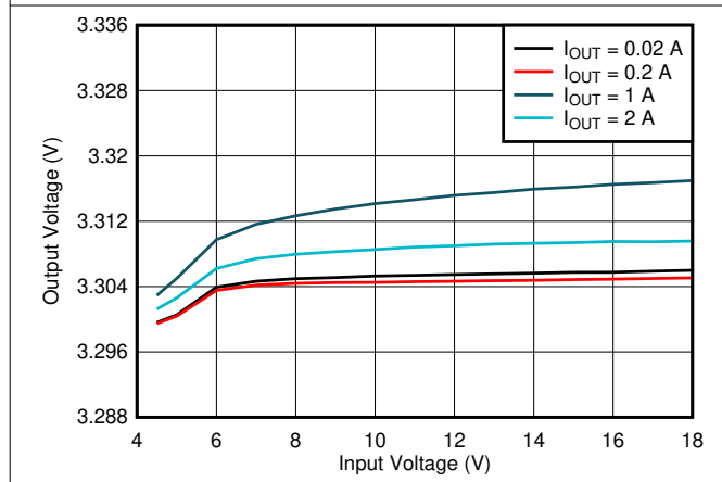
Figure 8-4. Line Regulation
