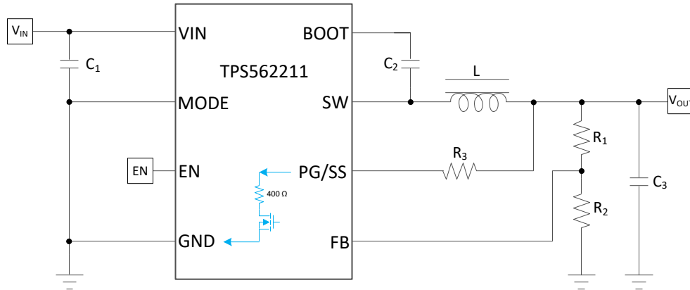
Figure 7-2. Discharge V OUT through PG/SS Pin with TPS562211
