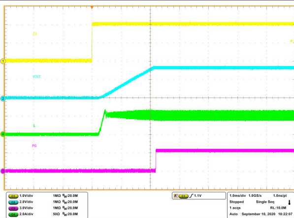
Figure 8-18. Enable Relative to EN
