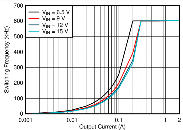
Figure 6-12. Switching Frequency vs Output Current, V_{OUT} = 3.3\text{ V} , L = 4.7\ \mu\text{H}
