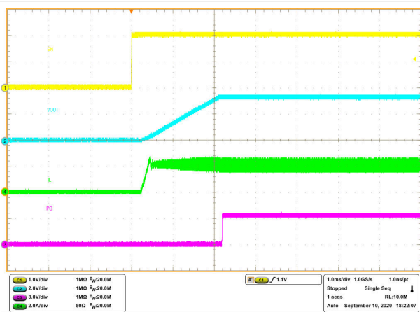
Figure 8-16. Enable Relative to EN
