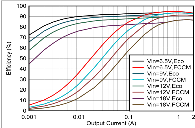
Figure 8-2. Efficiency
