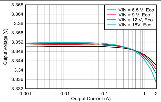
Figure 8-3. Load Regulation
