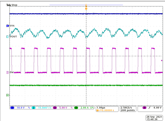
Figure 8-9. Steady State Waveforms, I_{OUT} = 2\text{ A}
