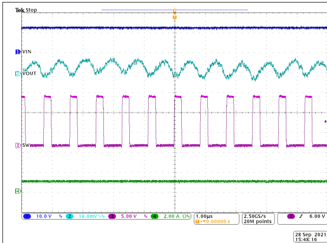
Figure 8-8. Steady State Waveforms, I_{OUT} = 1.0\text{ A}
