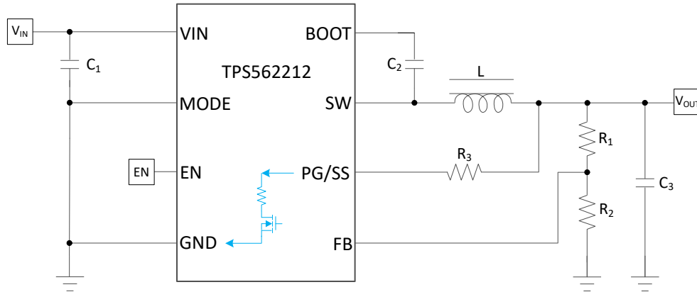
Figure 7-2. Discharge V OUT Through PG/SS Pin with TPS562212
