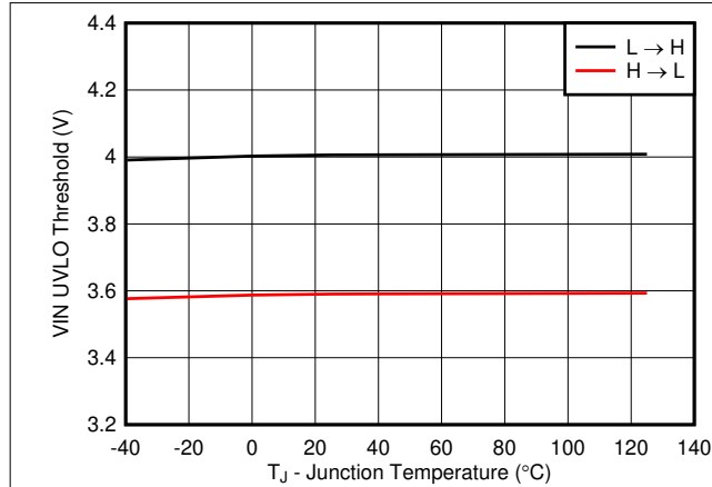
Figure 6-7. VIN UVLO Threshold vs Junction Temperature
