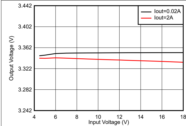
Figure 8-4. Line Regulation
