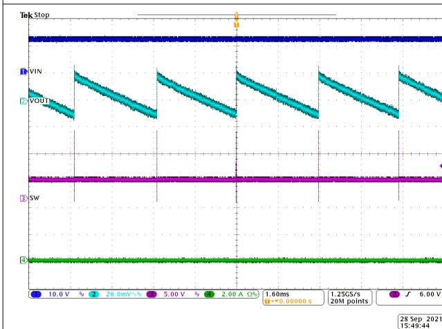
Figure 8-6. Steady State Waveforms, I_{OUT} = 0\text{ A}
