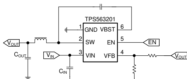
Simplified Schematic
