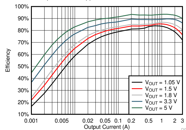
TPS563201 Efficiency
