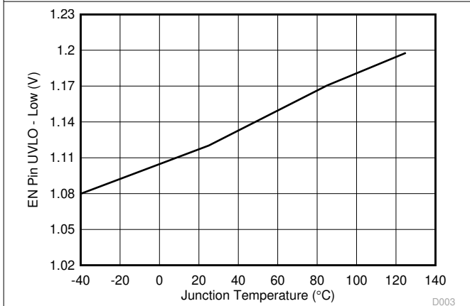
Figure 5-3. EN Pin UVLO Low Voltage vs Junction Temperature
