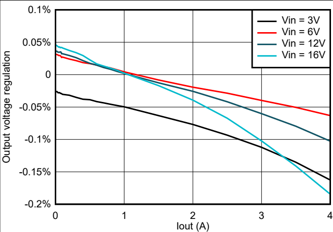
Figure 8-5. TPS564247 Load Regulation vs Loading
