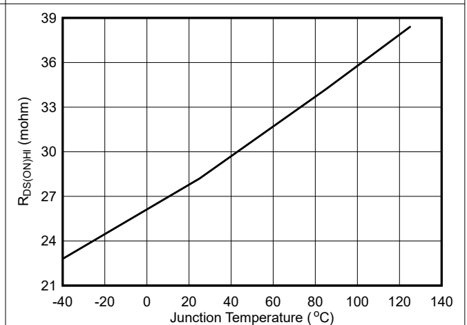
Figure 6-6. High-Side R_{DS(ON)}
