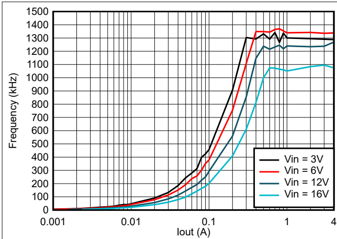
Figure 8-2. TPS564242 Frequency vs Loading
