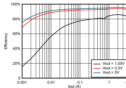
TPS564242 Efficiency at V_{IN} = 12 V
