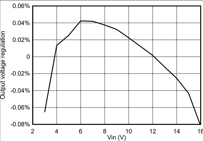
Figure 8-7. TPS564247 Line Regulation vs V_{IN} with 4-A Loading
