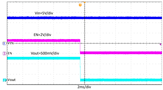
Figure 7-19. Shutdown Through EN, I OUT = 4A
