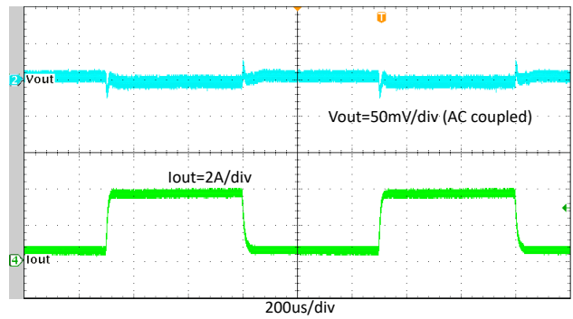
Figure 7-17. TPS564255B Transient Response With 0.4A to 3.6A
