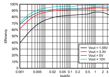
TPS564252B Efficiency at V_{IN} = 12\text{V}
