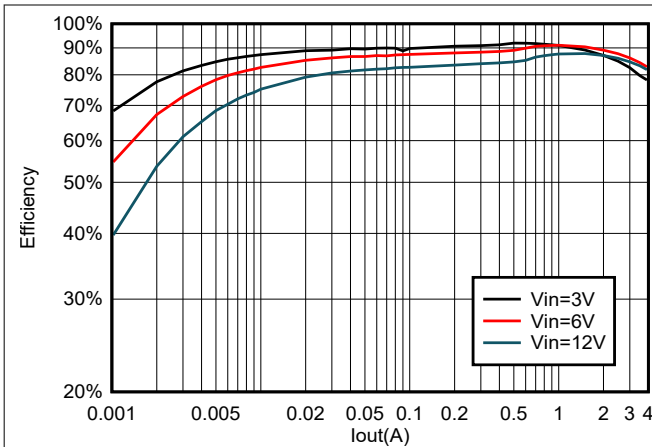
Figure 5-13. TPS564252B Efficiency at 1.05 V_{OUT} With a 1.5 \mu\text{H} Inductor
