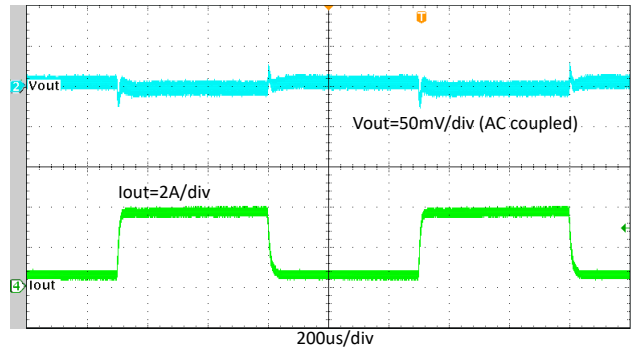
Figure 7-15. TPS564252B Transient Response With 0.4A to 3.6A
