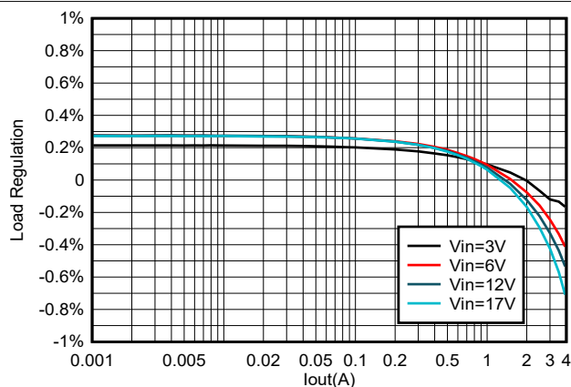
Figure 7-7. TPS564255B Load Regulation vs Loading
