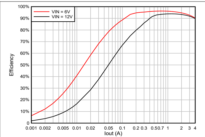
Figure 5-26. TPS564257C Efficiency at 3.3V OUT With a 2.2µH Inductor
