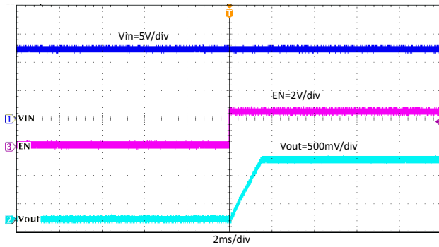
Figure 7-18. Start-up Through EN, I OUT = 4A
