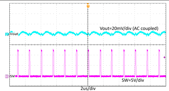
Figure 7-12. TPS564257B Output Voltage Ripple With 0.01A Loading
