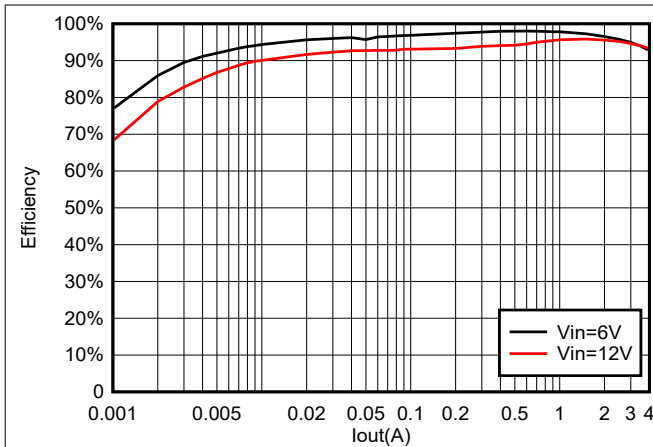
Figure 5-19. TPS564252B Efficiency at 5 V_{OUT} With a 4.7 \mu\text{H} Inductor
