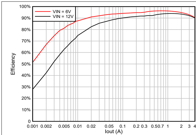
Figure 5-25. TPS564252C Efficiency at 3.3V OUT With a 2.2µH Inductor
