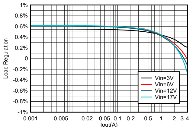
Figure 7-5. TPS564252B Load Regulation vs Loading
