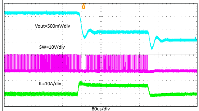
Figure 8-19. TPS565242 Normal Operation to Output Hard Short
