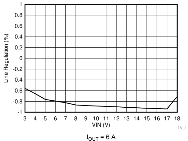
Figure 7-11. Line Regulation
