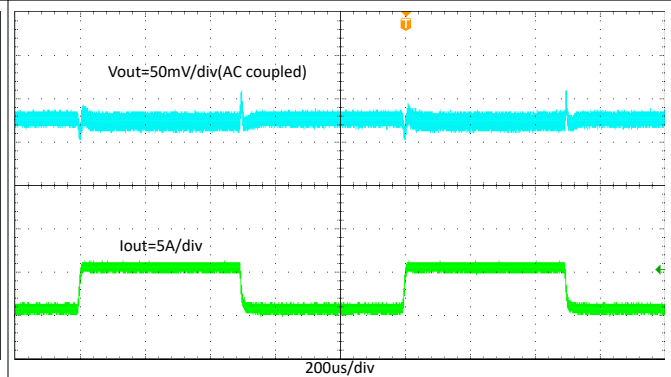
Figure 8-17. TPS566247 Transient Response with 0.6 A to 5.4 A by 2.5-A/ \mu\text{s} Load Step
