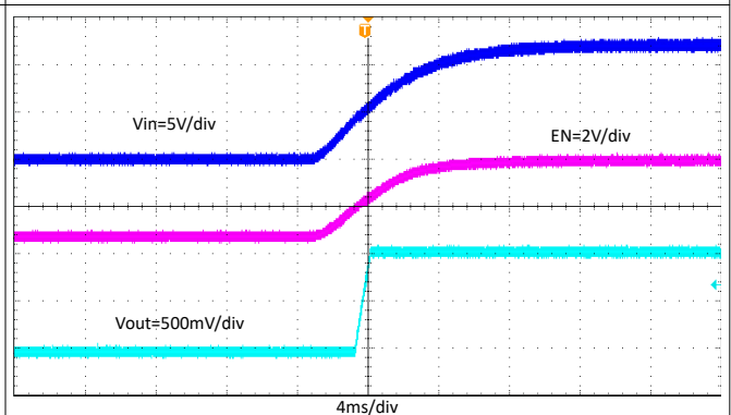
Figure 8-13. Start-Up with V_{IN} Rising, I_{OUT} = 6 A
