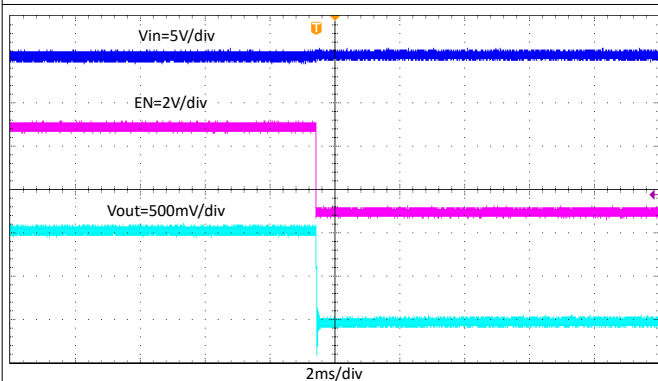
Figure 8-12. Shutdown Through EN, I_{OUT} = 6 A
