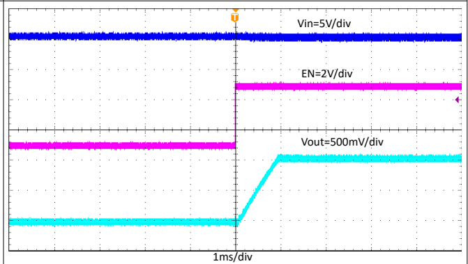
Figure 8-11. Start-Up Through EN, I_{OUT} = 6 A
