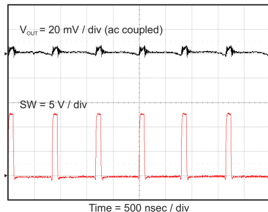
Figure 7-13. Output Voltage Ripple, I_{OUT} = 12 \text{ A}
