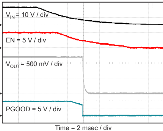
Figure 7-16. Shut Down Relative to V_{IN} Falling
