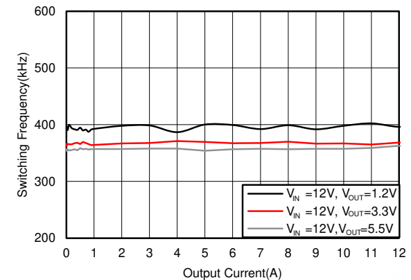
Figure 5-24. F_{SW} Load Regulation, Mode = FCCM, F_{SW} = 400 kHz
