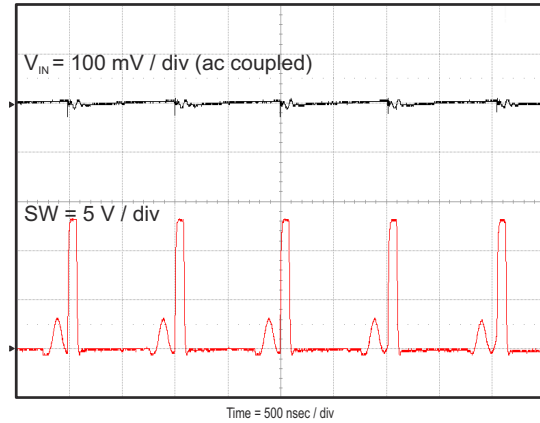
Figure 7-9. Input Voltage Ripple, I_{OUT} = 800 \text{ mA}
