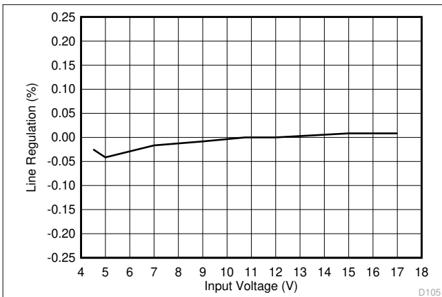
Figure 7-6. Line Regulation, I_{OUT} = 6\text{ A}
