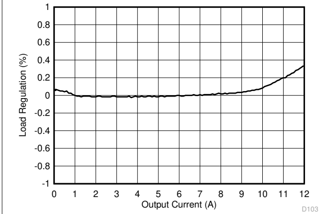
Figure 7-4. Load Regulation, V_{IN} = 5\text{ V}
