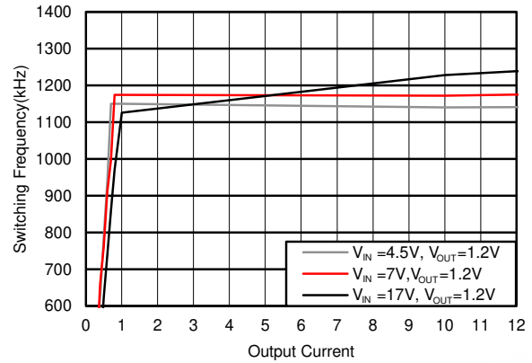
Figure 5-20. F_{SW} Load Regulation, Mode = DCM, F_{SW} = 1200 kHz
