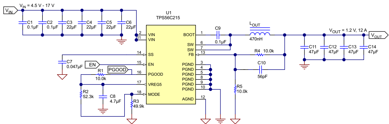
Figure 7-1. Application Schematic
