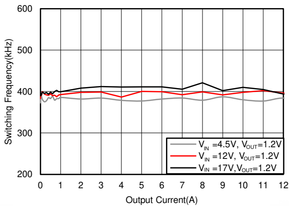
Figure 5-21. F_{SW} Load Regulation, Mode = FCCM, F_{SW} = 400 kHz
