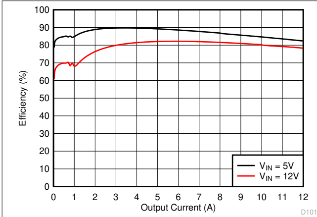
Figure 7-2. Efficiency
