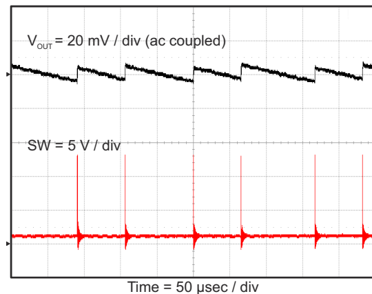
Figure 7-11. Output Voltage Ripple, I_{OUT} = 10 \text{ mA}
