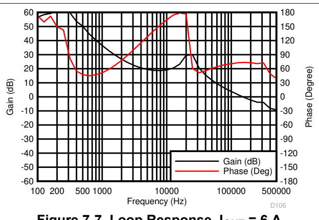
Figure 7-7. Loop Response, I_{OUT} = 6\text{ A}
