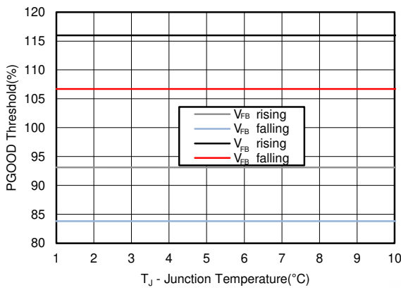
Figure 5-9. PGOOD Threshold vs Temperature
