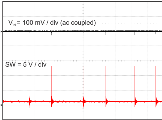
Figure 7-8. Input Voltage Ripple, I_{OUT} = 10 \text{ mA}
