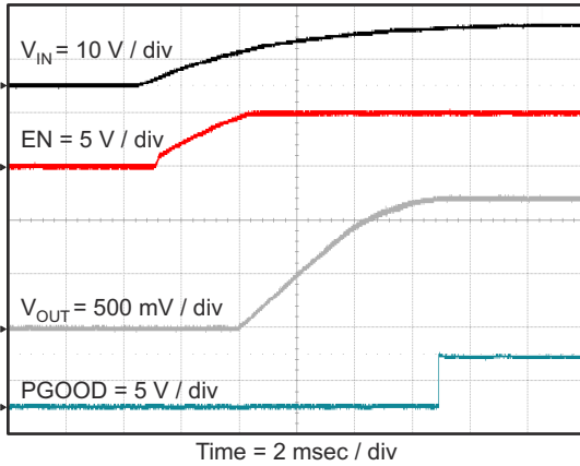
Figure 7-14. Start Up Relative to V_{IN} Rising
