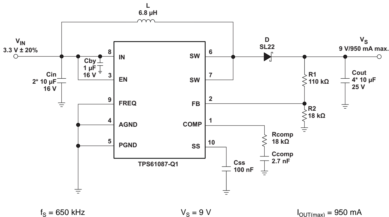
Figure 16. 3.3-V to 9-V Application Diagram
