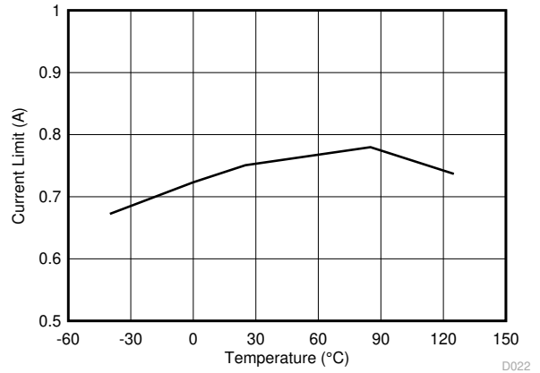
TPS613223A L = 4.7 μH
