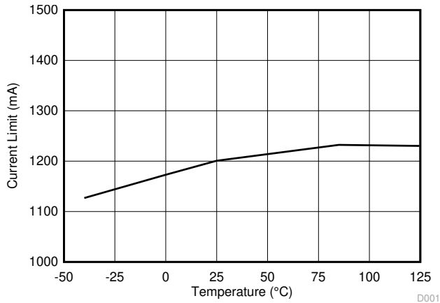
TPS613226A L = 2.2 μH
