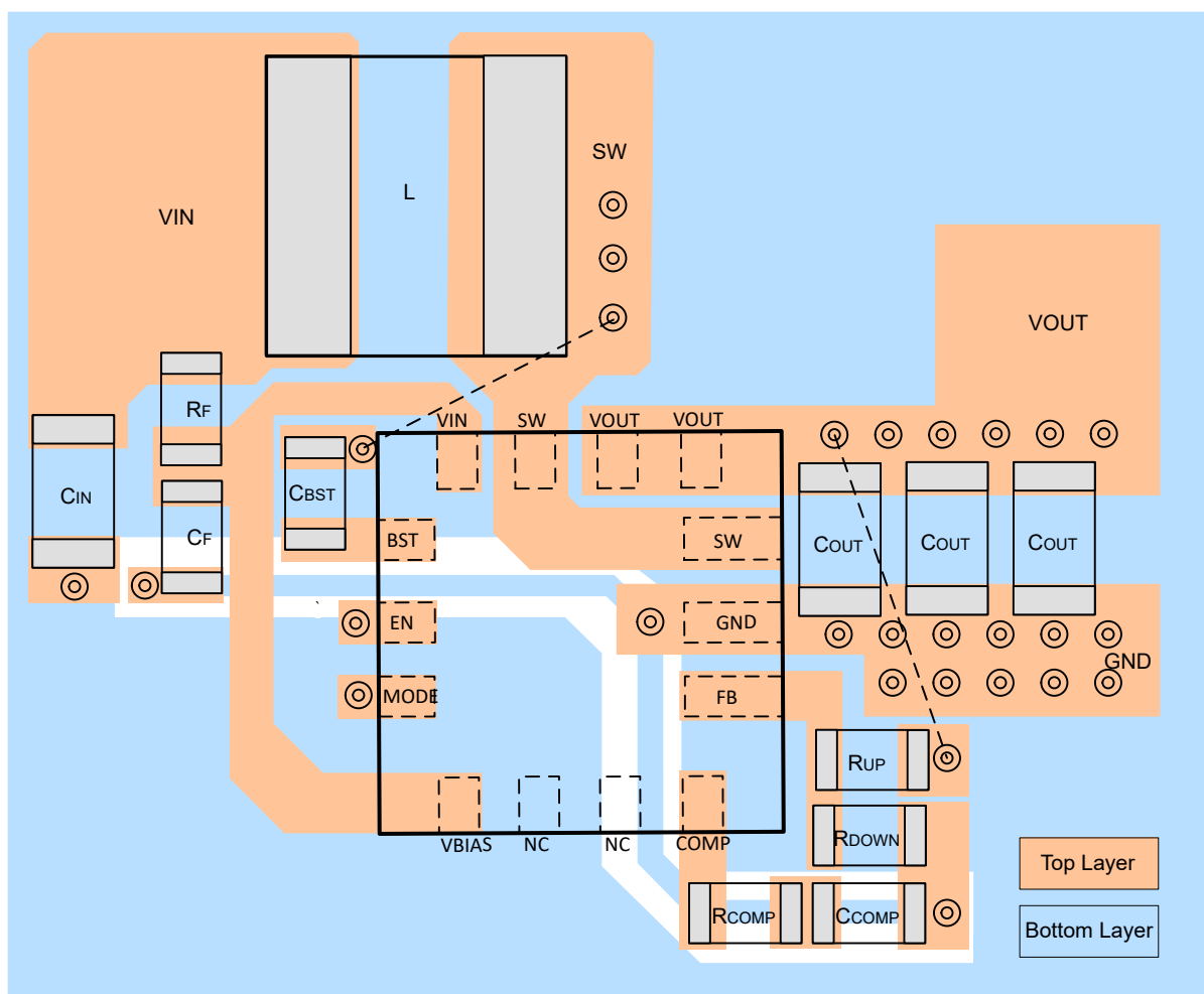
Figure 7-9. Recommended Layout
