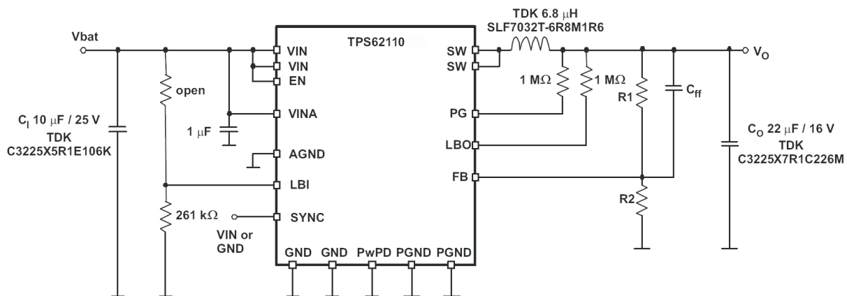
Figure 9. Test Setup
