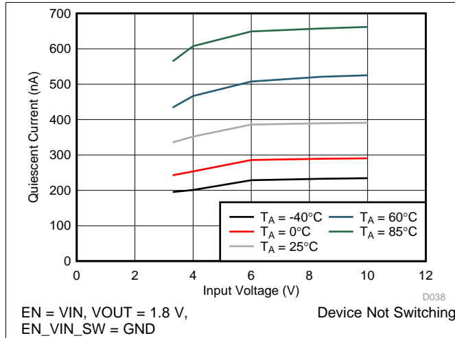
Figure 1. Quiescent Current
