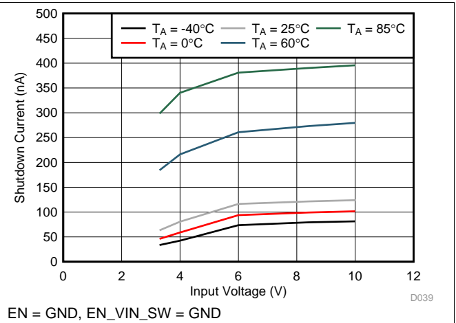
Figure 2. Shutdown Current
