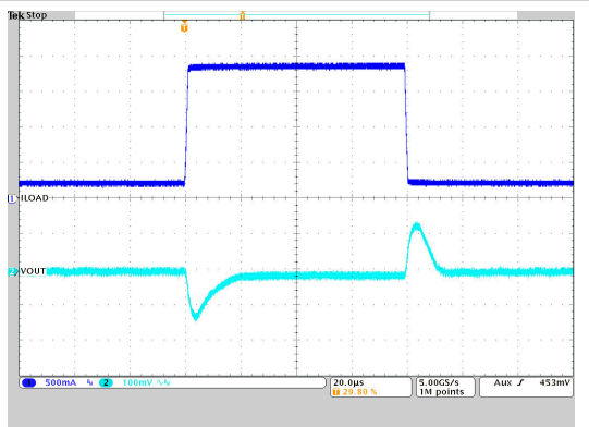
Figure 9-24. Load Transient Response
