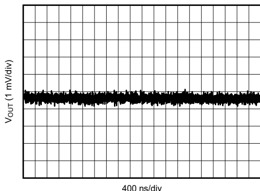
Figure 5-11. V_{OUT} Ripple After the Second L-C Filter
