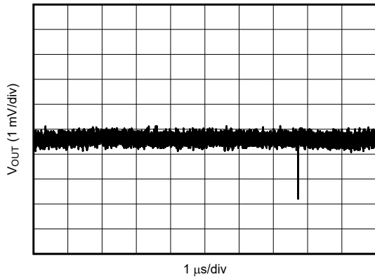
Figure 5-7. V_{OUT} Ripple After the Second L-C Filter
