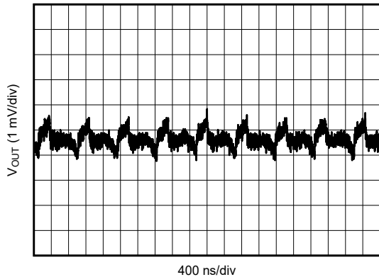
Figure 5-9. V_{OUT} Ripple After the First L-C Filter
