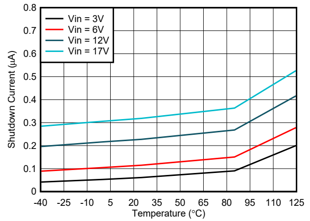
Figure 7-2. Typical Shutdown Current vs Temperature
