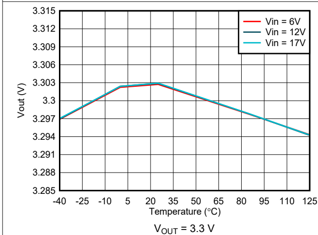
Figure 7-5. Output Voltage Accuracy – VSET Selected
