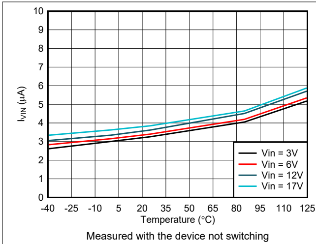
Figure 7-1. Typical Quiescent Current vs Temperature
