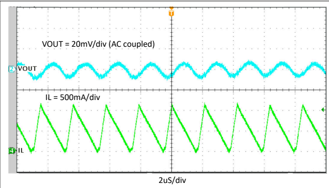
Figure 10-15. Steady State, I_{OUT} = 0.5 \text{ A}
