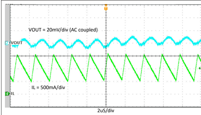
Figure 10-16. Steady State, I_{OUT} = 1 \text{ A}
