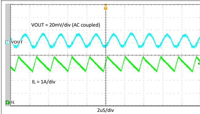
Figure 10-18. Steady State, I_{OUT} = 3 \text{ A}
