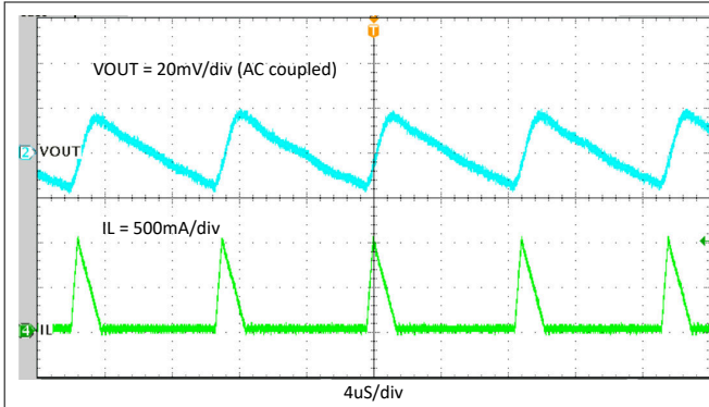
Figure 10-14. Steady State, I_{OUT} = 0.1 \text{ A}
