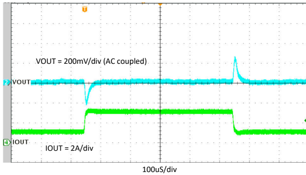
Figure 10-20. Load Transient Response, 1 to 3 A, Slew Rate = 0.8 A/ \mu S
