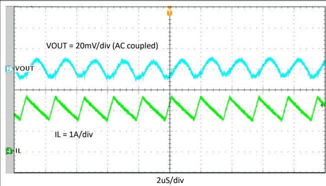
Figure 10-17. Steady State, I_{OUT} = 2 \text{ A}
