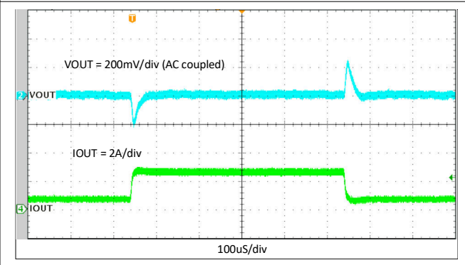
Figure 10-19. Load Transient Response, 0.5 to 2.5 A, Slew Rate = 0.8 A/ \mu\text{S}
