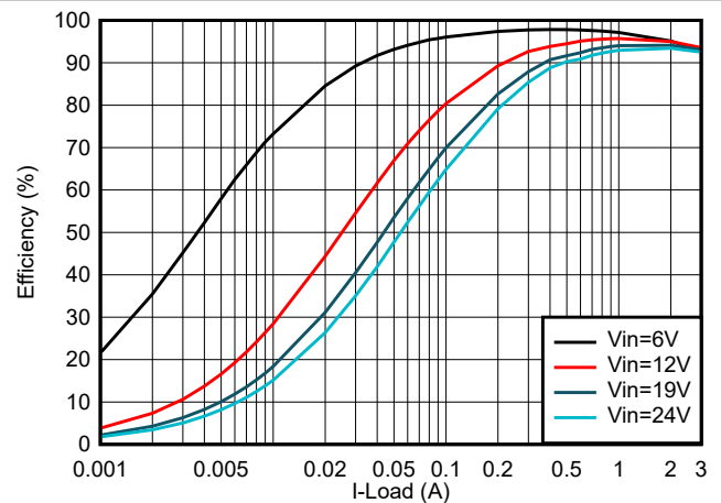
Figure 8-22. TPS62933F Efficiency, V_{OUT} = 5\text{ V} , f_{SW} = 500\text{ kHz} , L = 6.8\ \mu\text{H}
