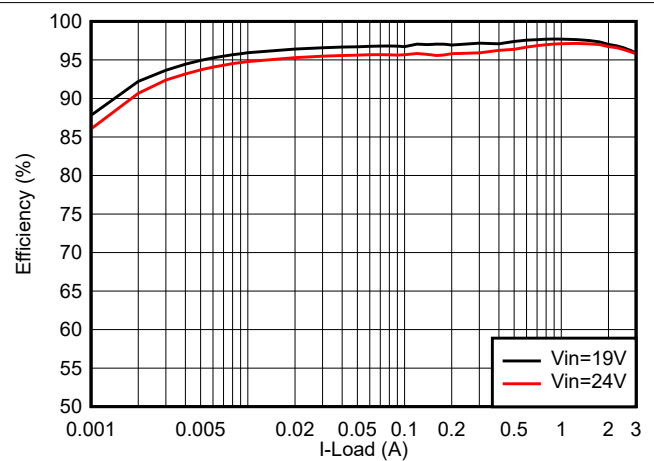
Figure 8-20. TPS62933 Efficiency, V_{OUT} = 12\text{ V} , f_{SW} = 500\text{ kHz} , L = 12\ \mu\text{H}
