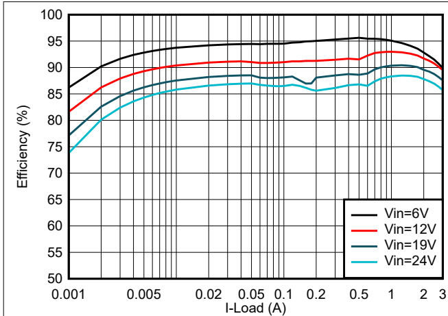
Figure 8-19. TPS62933 Efficiency, V_{OUT} = 3.3\text{ V} , f_{SW} = 1200\text{ kHz} , L = 2.2\ \mu\text{H}
