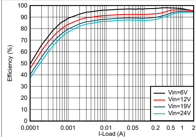
Figure 8-21. TPS62932 Efficiency, V_{OUT} = 5\text{ V} , f_{SW} = 500\text{ kHz} , L = 10\ \mu\text{H}
