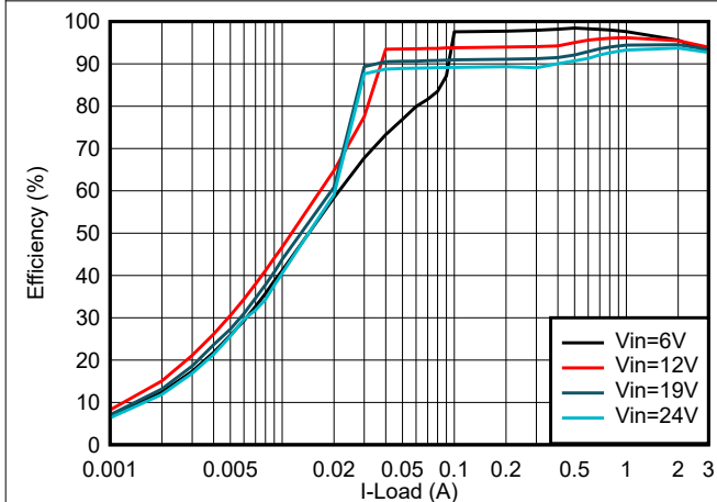
Figure 8-23. TPS62933O Efficiency, V_{OUT} = 5\text{ V} , f_{SW} = 500\text{ kHz} , L = 6.8\ \mu\text{H}
