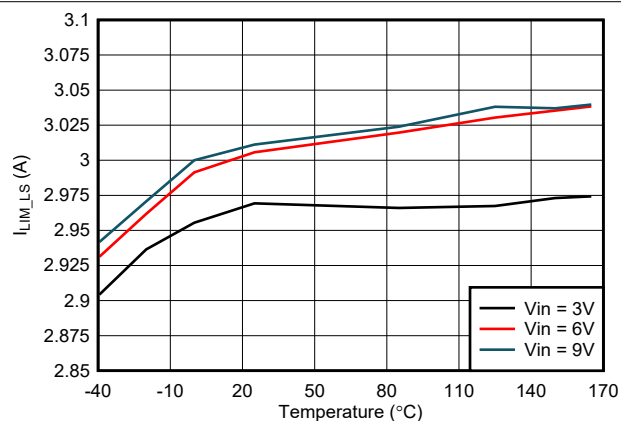
Figure 7-16. Low Side I_{LIM} vs Temperature
