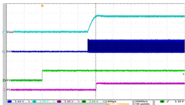
Figure 9-65. Start-Up Timing
