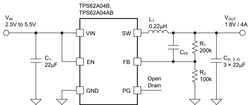
Figure 8-1. TPS62A04xB Typical Application Circuit
