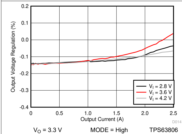
Figure 10-23. Load Regulation (PWM Only)
