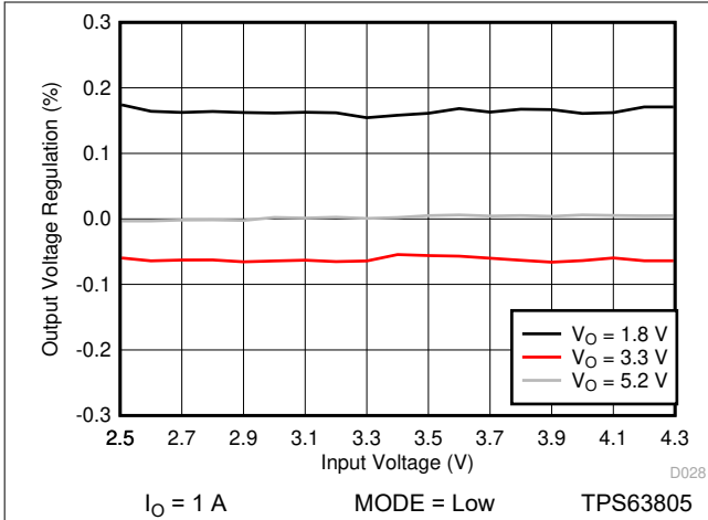
Figure 10-21. Line Regulation (PWM Only)
