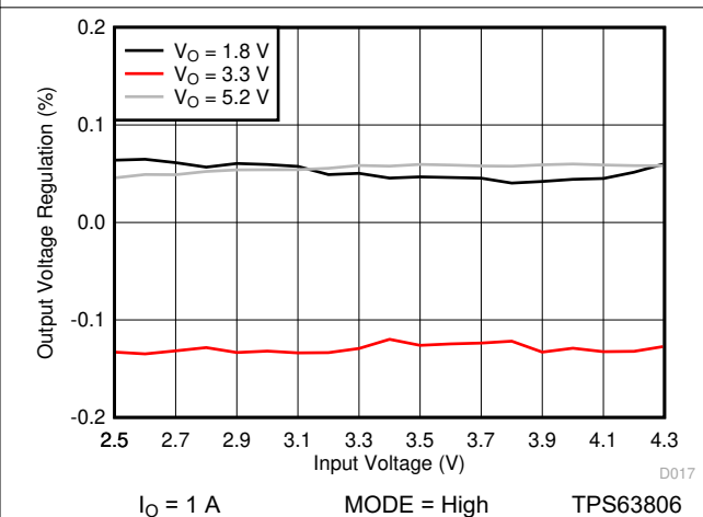
Figure 10-26. Line Regulation (PFM/PWM)
