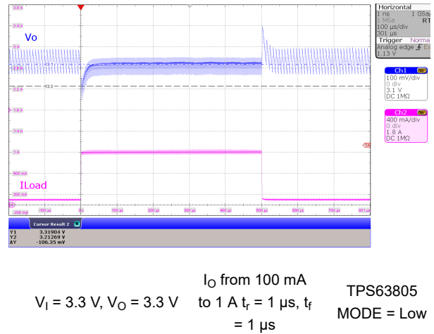
Figure 10-34. Load Transient, PFM/PWM Buck-Boost Operation
