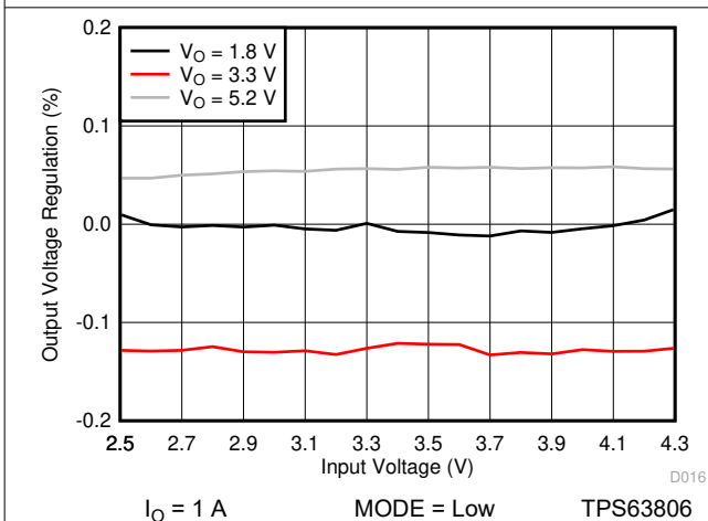
Figure 10-25. Line Regulation (PWM Only)
