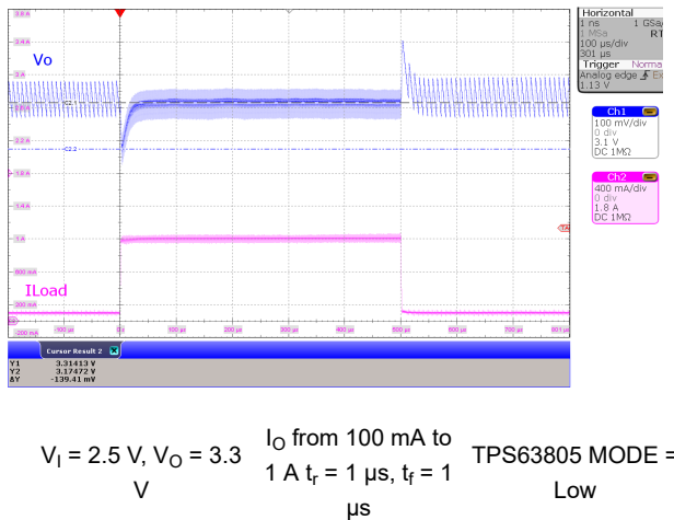
Figure 10-33. Load Transient, PFM/PWM Boost Operation
