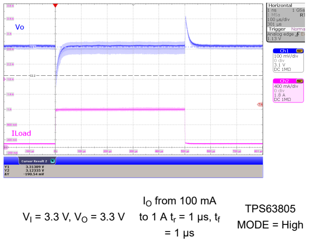
Figure 10-37. Load Transient, PWM Buck-Boost Operation
