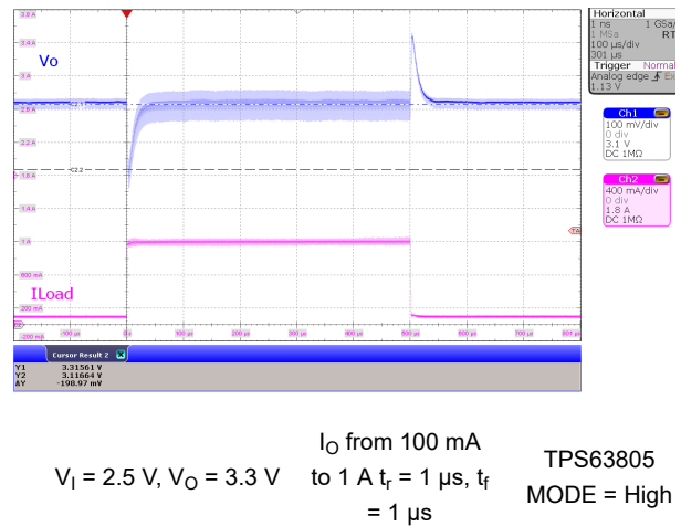
Figure 10-36. Load Transient, PWM Boost Operation
