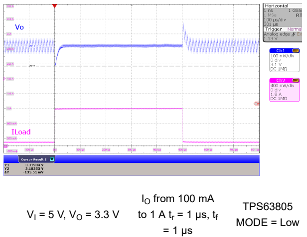
Figure 10-35. Load Transient, PFM/PWM Buck Operation
