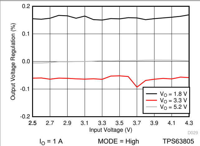
Figure 10-22. Line Regulation (PFM/PWM)
