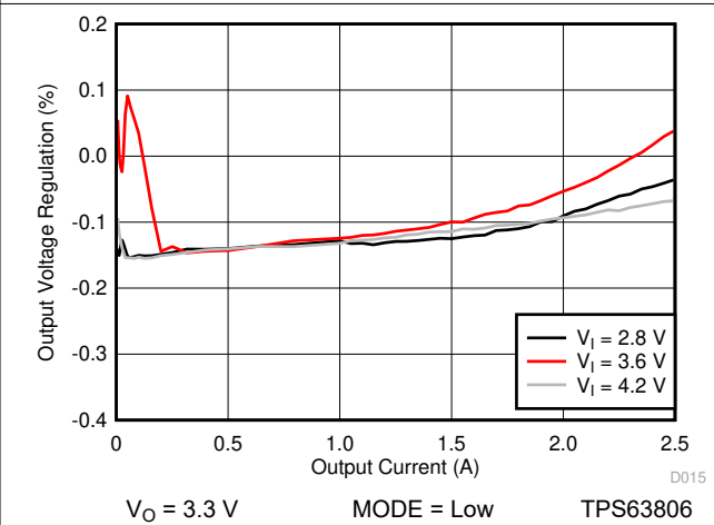
Figure 10-24. Load Regulation (PFM/PWM)
