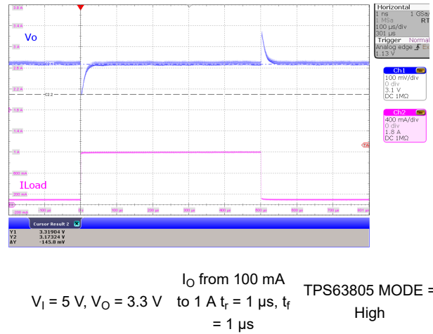
Figure 10-38. Load Transient, PWM Buck Operation
