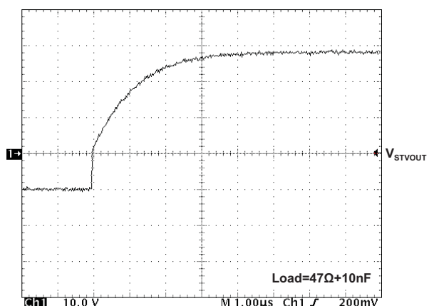
RISE TIME (STVOUT, RESETOUT)
