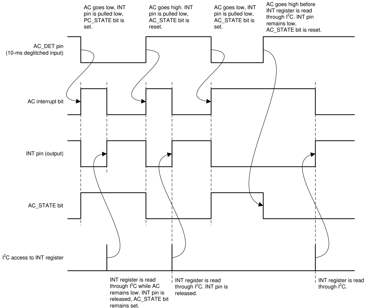
Figure 6-19. AC_STATE Pin
