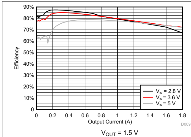
Figure 8-4. DCDC3 Efficiency
