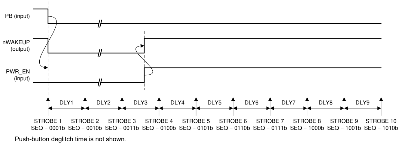
Figure 6-1. Power-Up Sequences from OFF or SUSPEND State; PB is Power-Up Event
