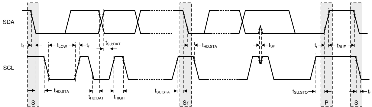
Figure 6-23. I 2 C Protocol and Transmission Timing I 2 C Data Transmission Timing
