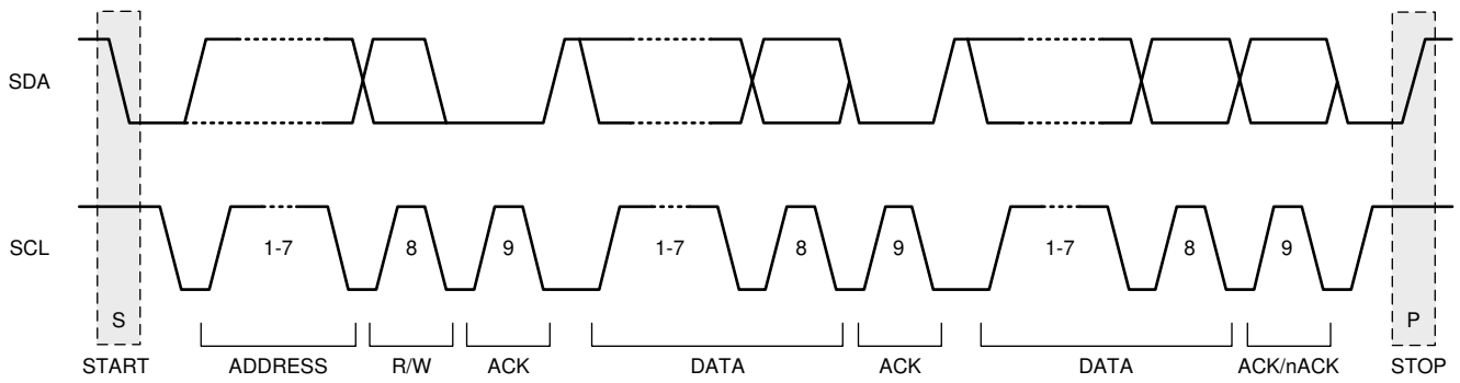
Figure 6-22. I 2 C Protocol and Transmission Timing I 2 C Start Stop and Acknowledge Protocol
