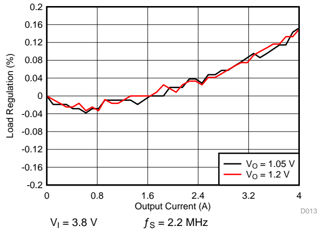
Figure 7-9. SMPS Load Regulation for 4-A Dual Phase
