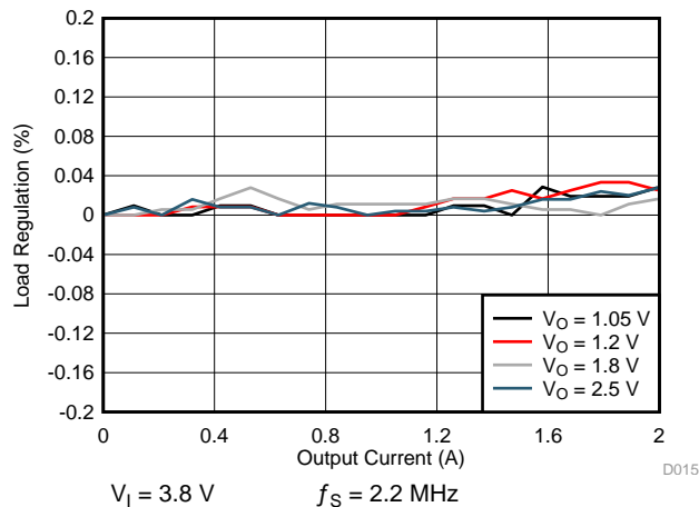
Figure 7-11. SMPS Regulation for 2-A Single Phase
