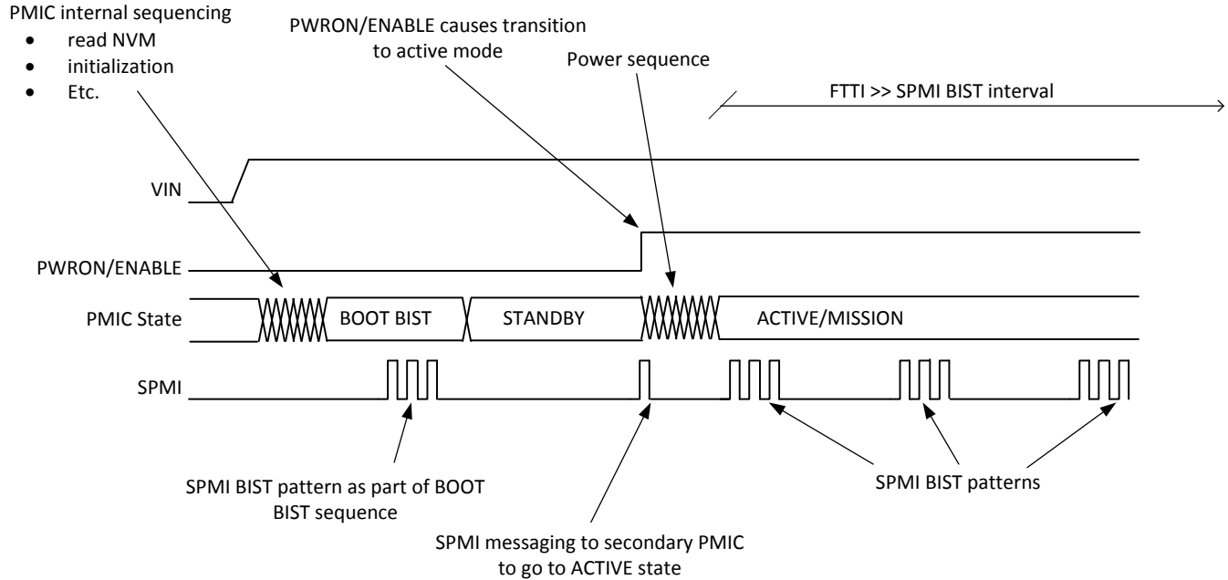
Figure 8-47. SPMI-BIST Operation
