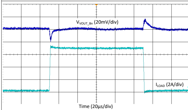
I_{LOAD} = 0.1\text{ A} \rightarrow 7\text{ A} \rightarrow 0.1\text{ A} , T_R = T_F = 1\mu s V_{PVIN\_Bn} = 3.3\text{ V} V_{VOUT\_Bn} = 1\text{ V} Figure 9-38. Buck Load Step Transient - 4-Phase, 2.2 MHz, Auto Mode
