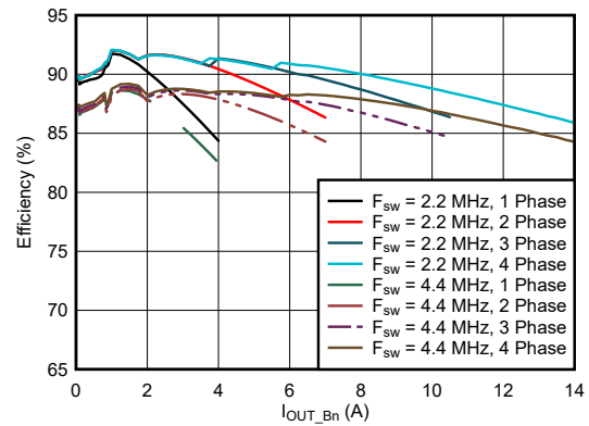
Figure 9-5. BUCK Efficiency with F_{sw} = 2.2\text{ MHz} or 4.4\text{ MHz}
