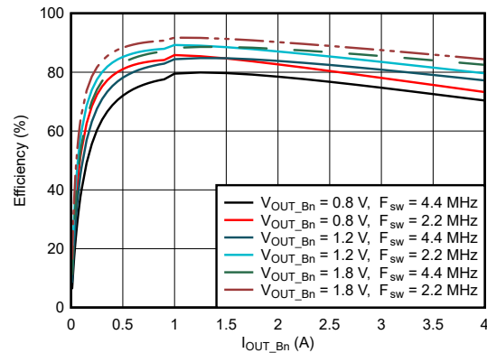
Figure 9-7. BUCK Efficiency in Varied Phase Configuration, 5 V Input
