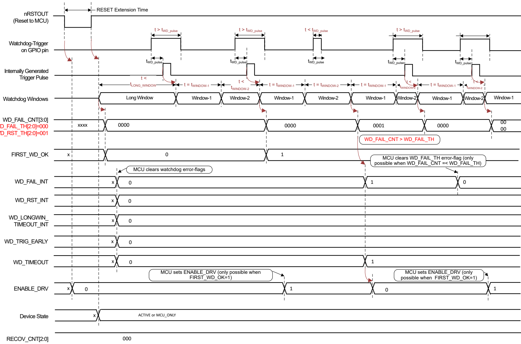
Figure 8-20. Watchdog in Trigger Mode – Good Events (Correct Watchdog-Triggers) After Start-up, Followed by a Bad-Event (No Watchdog-Triggers in Window-2) and After That Followed by a Good Event.
