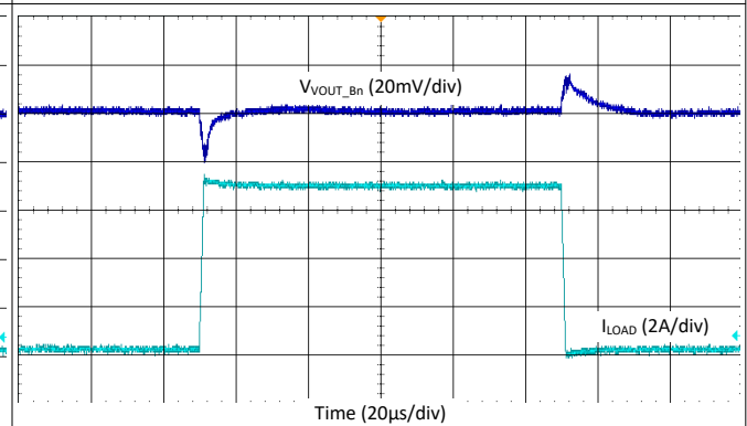
I_{LOAD} = 0.1\text{ A} \rightarrow 7\text{ A} \rightarrow 0.1\text{ A} , T_R = T_F = 1\mu s V_{PVIN\_Bn} = 3.3\text{ V} V_{VOUT\_Bn} = 1\text{ V} Figure 9-39. Buck Load Step Transient - 4-Phase, 4.4 MHz, Auto Mode
