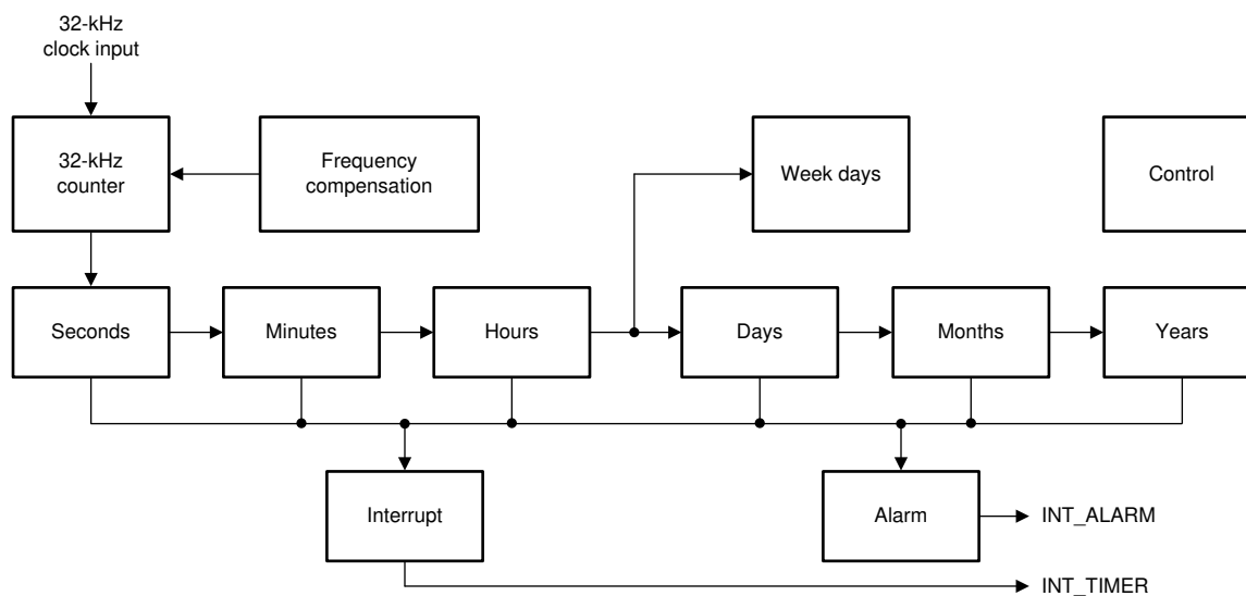
Figure 8-13. RTC Block Diagram
