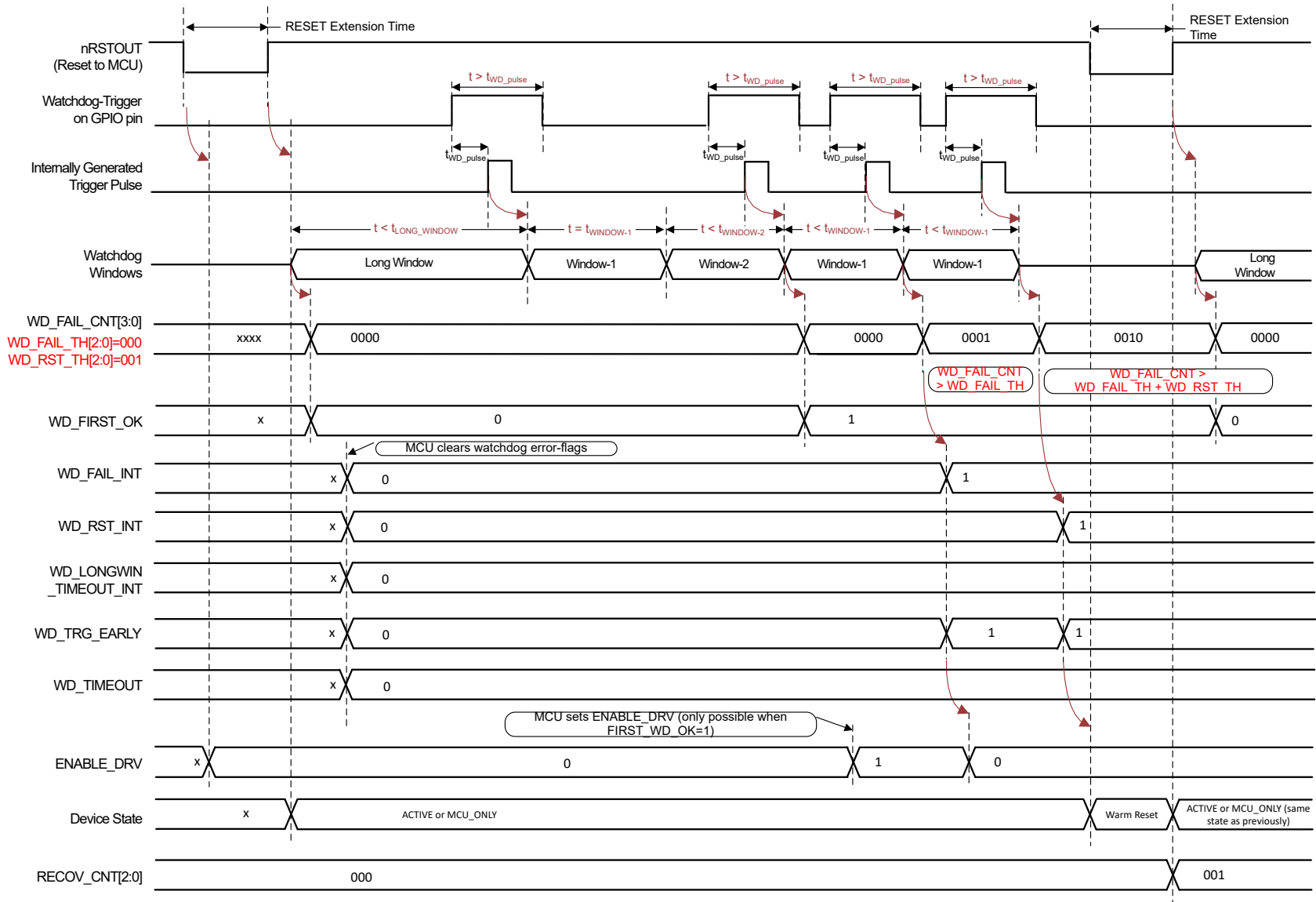
Figure 8-18. Watchdog in Trigger Mode – Bad Event (Watchdog-Triggers in Window-1) After Start-up
