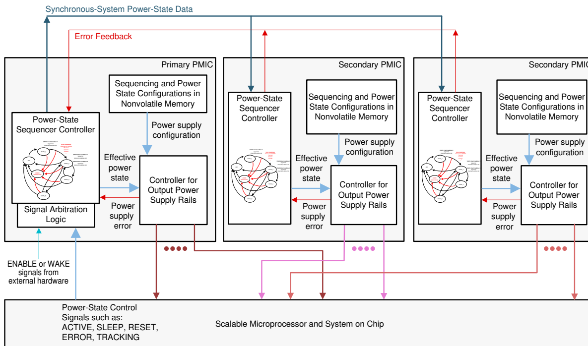
Figure 8-43. Multi-PMIC Power State Synchronization Block Diagram
