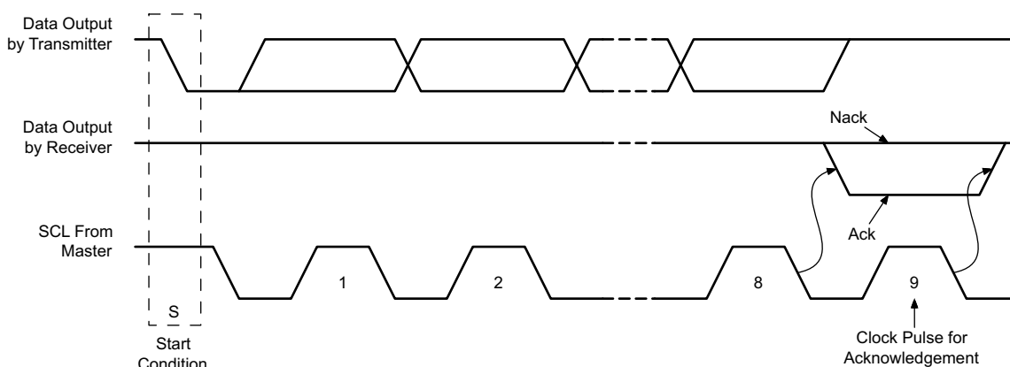
Figure 8-24. I²C Acknowledgment
