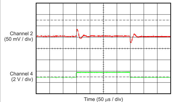
Figure 5-34. TPS70933-Q1 Load Transient (50 mA to 150 mA)
