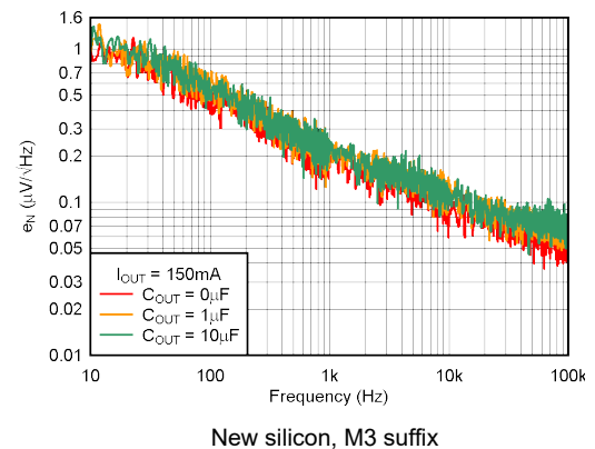
Figure 5-30. Noise Spectral Density C_{NR} = 0.01\ \mu\text{F}
