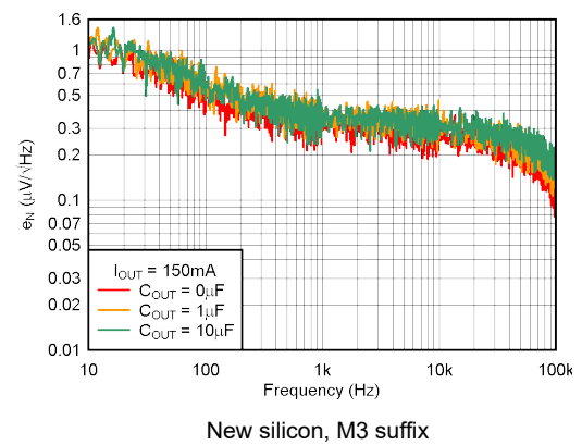
Figure 5-28. Noise Spectral Density C_{NR} = 0\ \mu\text{F}
