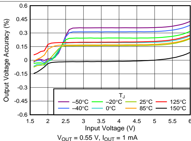
Figure 2. 0.55-V Line Regulation vs V_{IN}
