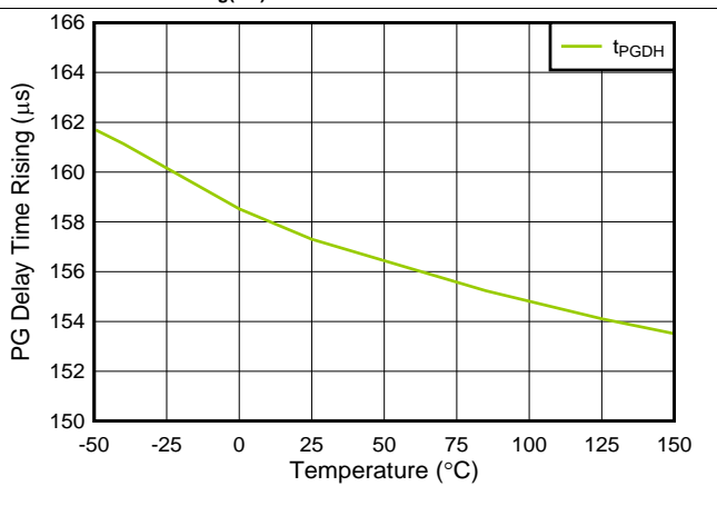
Figure 18. t_{PGDH} vs Temperature
