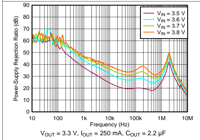
Figure 33. PSRR vs Frequency and V_{IN}
