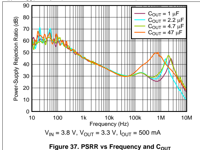
Figure 37. PSRR vs Frequency and C_{OUT}
