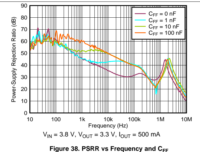
Figure 38. PSRR vs Frequency and C_{FF}
