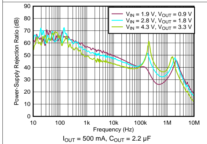
Figure 35. PSRR vs Frequency
